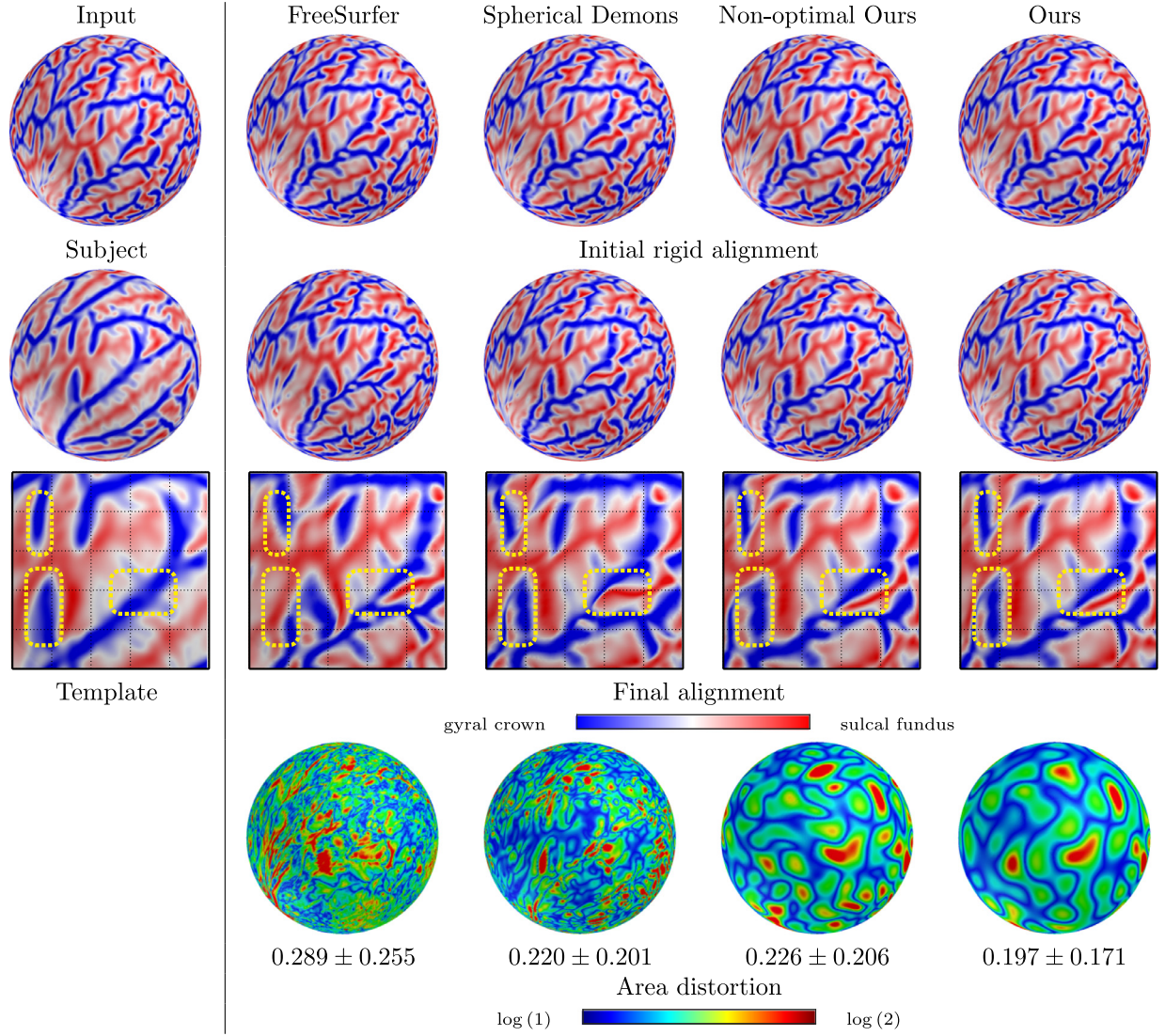
Fig. 6. An example of pair-wise registration from a single subject to a fixed template. These methods begin with almost the same rigid alignment before the local deformation and produce similar hCuv patterns with slight difference. However, FreeSurfer and Spherical Demons only update the local deformation during the optimization. This results in relatively large deformation in several regions, whereas the proposed method updates both rigid and non-rigid deformation to reduce locally focused deformation. Also, the optimal rigid alignment in our method provides improved feature alignments and registration distortion compared to ours with a non-optimal rigid alignment.
