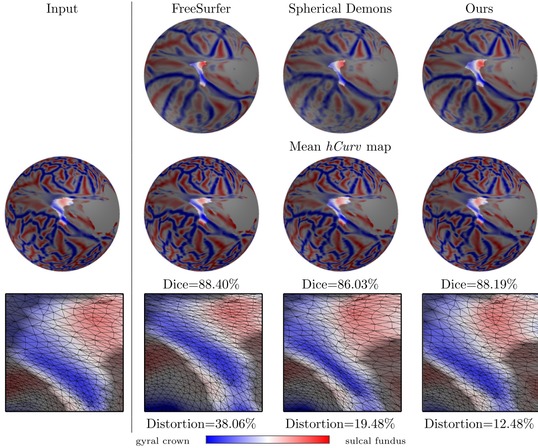
Fig. 15. An example area change in Ent. (top) The three methods yield similar cortical folding patterns after co-registration (see Fig. 7 for the average hCurv maps). The mode regions of Ent are highlighted brightly. (middle) The Dice coefficients are comparable, which implies that these methods achieve comparable performance in surface alignment; the hCurv maps are also well aligned with the averages. (bottom) Even with comparable registration performance, the surface area (triangle size) is less distorted in the proposed method than FreeSurfer and Spherical Demons. It is noteworthy that the mode region of Ent in our group-wise framework is little larger than others because the distortion can be better minimized (i.e., better area preservation) in this way, while maintaining comparable registration accuracy (see Fig. 9 for Ent).
