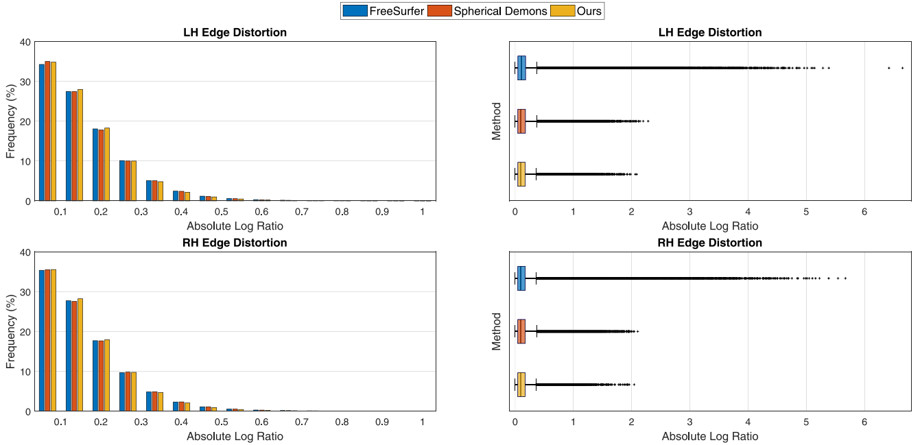
Fig. 12. Edge distortion (whiskers with maximum 1.5 interquartile range). The proposed method has a less skewed distribution to the right (shorter tail). This implies a fewer number of regions with large edge distortion than FreeSurfer and Spherical Demons on both hemispheres.
