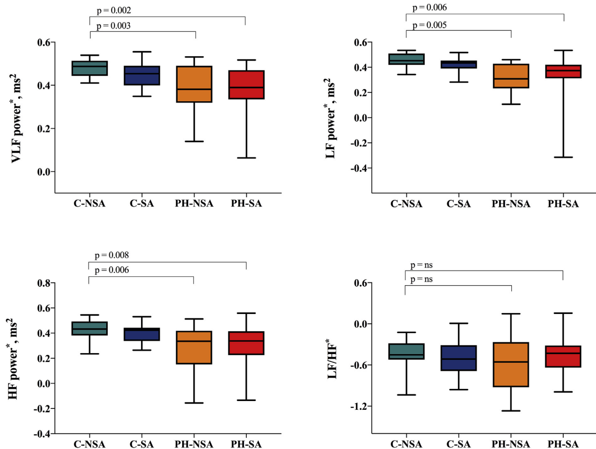
Fig. 2. Frequency domain HRV analysis. Box and whisker plots of HRV in control and PH subjects both with and without SA. Abbreviations: HRV = heart rate variability, C = Control, NSA = no sleep apnea, SA = sleep apnea, PH = pulmonary hypertension, VLF = very low frequency, LF = low frequency, HF = high frequency, LF/HF = low frequency/high frequency ratio. Box and whisker plots presented as median (p5–p95). * Log 10 .
