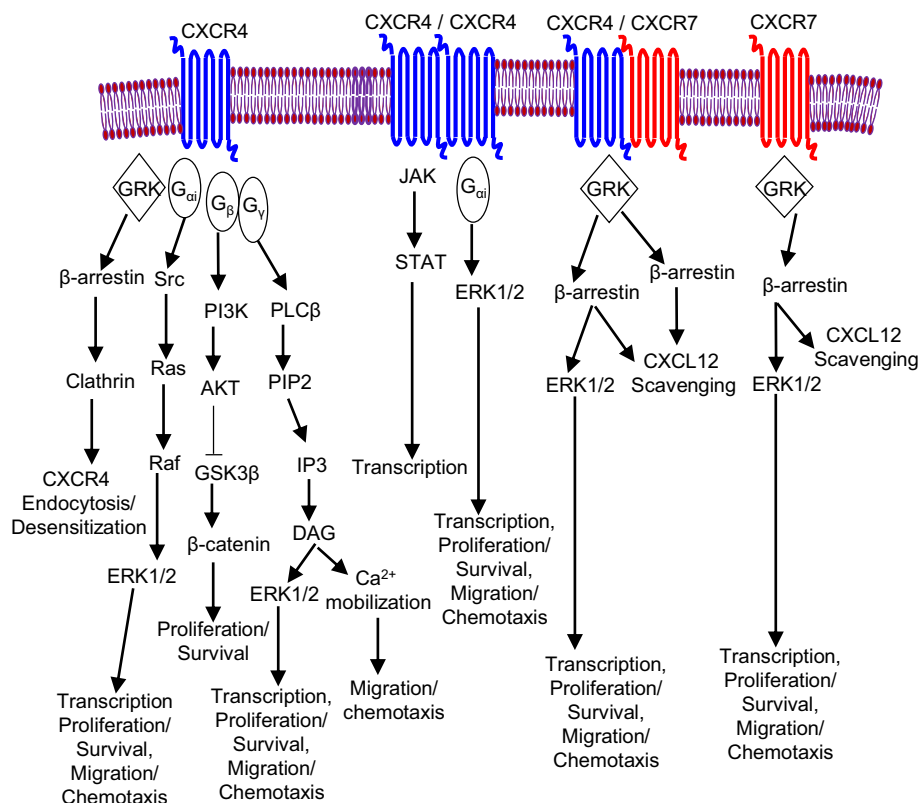
Fig. 1. CXCL12/CXCR4/CXCR7 signaling CXCL12 acts on CXCR4 and CXCR7, which are two distinct seven-membrane transpanning G-protein-coupled receptors. CXCR4 can transduce signaling as a monomer, homodimer or heterodimer with CXCR7. Binding of CXCL12 to CXCR4 can transduce classical G-protein-coupled signaling to activate ERK1/2, PI3K/AKT, PLCB/IP3 pathways, culminating in cell proliferation/survival and migration/chemotaxis or gene transcription. Activated homodimers of CXCR4 can transduce JAK/STAT signaling independent of G-protein and subsequent gene transcription as well as G-protein-coupled signaling and subsequent ERK1/2 pathways. Heterodimerization of CXCR4 with CXCR7 preferentially elicits \beta -arrestin-mediated signaling to activate ERK1/2 signaling or result in CXCL12 scavenging. CXCR7 transduces CXCL12-mediated signaling via \beta -arrestin independent of G-protein and activates ERK1/2 signaling or CXCL12 scavenging.
