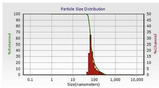
(E) DLS spectrum of AgNPs of A. marmelos methanolic extract
