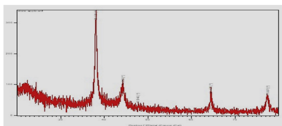
(C) XRD pattern of AgNPs of A. marmelos methanolic extract
