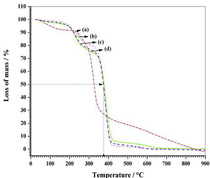
Figure 3. TGA curves demonstrating the weight loss of polymer materials during heating ( A ) α-GOS, (b) isolated Standard Film (Eudragit® RS30D + 20% TEC), (c) isolated Film 95:05 (Standard +5% of α-GOS) and (d) isolated Film 90:10 (Standard +10% of α-GOS).
