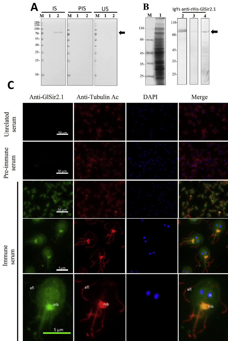
Fig. 5. GISir2.1 of G. lamblia is a cytoplasmic protein. A: Evaluation of the obtained sera against 100 ng of the recombinant protein rHis-GISir2.1 and 100 ng of BSA. IS: immune serum anti-rHis-GISir2.1, dilution 1/5000. PIS: pre-immune serum, dilution 1:5000. US: unrelated serum, dilution 1:5000. (1); 100 ng of BSA. (2); 100 ng of rHis-GISir2.1. (M); Pre-stained molecular weight marker, in kDa. B: Detection of the endogenous Giardia lamblia Sir2.1. SDS-PAGE- Coomassie. (M); Molecular weight marker, in kDa. (1); Total protein extracts of Giardia trophozoites ( 1 \times 10^6 cells). Western blot. (2); 50 ng of rHis-GISir2.1, dilution 1:250 of IgYs anti-rHis-GISir2.1. (3–4); total protein extracts ( 1 \times 10^6 cells), dilution 1:500 and 1:250 of IgYs anti-rHis-GISir2.1. Black arrow indicates the rHis-GISir2.1 or the endogenous protein. C: The unrelated, pre-immune and immune sera were employed in an indirect immunofluorescence assay with G. lamblia trophozoites. Green: endogenous GISir2.1 localization. Red: acetylated alpha tubulin localization. Blue: nucleus localization (DAPI). White bars: 50 \mu m. Green bar: 5 \mu m. afl: anterior flagella. mb: Median body.
