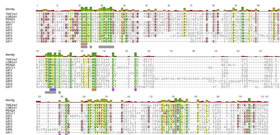
Fig. 1. The primary structure of the G1Sir2.1 protein shows conserved characteristics of the sirtuin family. Multiple sequence alignment of G1Sir2.1 N-terminal domain with human sirtuins (SIRT1-7), TbSir2rp1 ( T. brucei ), PfsIR2A ( P. falciparum ), and LiSIR2rp1 ( L. infantum ). The highly conserved predicted NAD + binding residues are in grey. Peach and blue: NAD + binding GAG and NVD motifs. Orange: HG motif. Pink: conserved zinc binding cysteine residues. The percentage of identity among sequences is proportional to the height of the bars. Color; Green: 100% similarity. Yellow: 80–90% similarity. Pink: 60–80% similarity. Without color: less of 60% similarity. The multiple sequence alignment was generated with T-COFFEE (Tommaso et al., 2011) and visualized using Geneious version 6.1.6 (Kearse et al., 2012).
