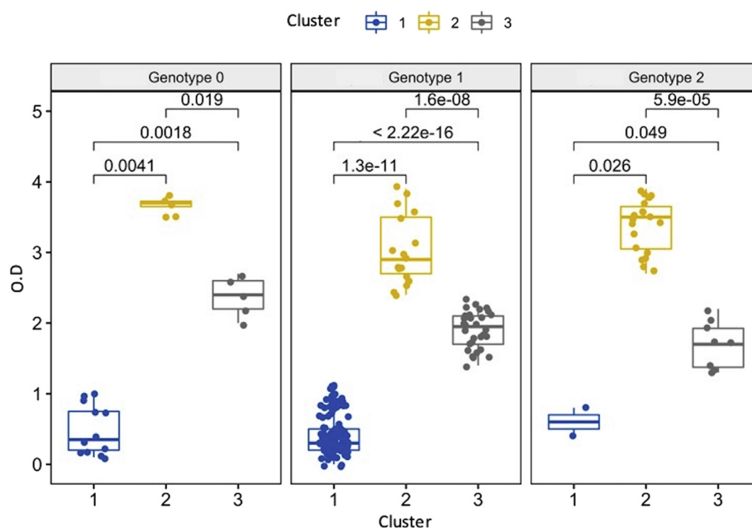
Fig. 3. Box plot of the distribution of the optical densities (OD) of S. aureus strains ( n = 229 ) recovered from IMI in Colombian dairy herds ( n = 91 ) by each cluster ( k = 3 ) and grouped by genotypes ( n = 3 ). Dots represent the specific observations by group of cluster and genotypes. Significant differences were presented as Pairwise unpaired comparisons Wilcoxon test P values. The box and blue dots represent cluster 1 ( n = 146 ; OD: \leq 1.1 ), yellow to cluster 2 ( n = 40 ; OD: \geq 2.4 ), and grey to cluster 3 ( n = 43 ; OD: 1.3\text{--}2.7 ). Most of the strains from genotype 1 (73.74%) and genotype 0 (57.14%) were classified into cluster 1, while a high percentage (65.51%) of isolates from genotype 2 were linked to cluster 2.
