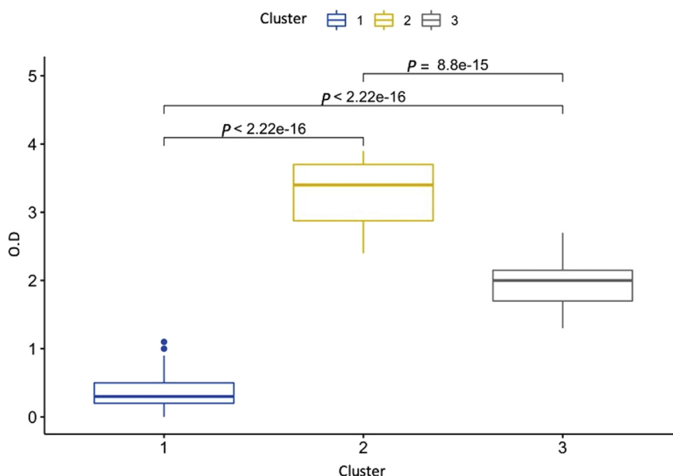
Fig. 2. Box plot representation of distribution of the optical densities (OD) of S. aureus strains ( n = 229 ) recovered from IMI in dairy herds ( n = 91 ) from Colombia grouped by clusters ( k = 3 ). The Kruskal-Wallis test showed significant differences among clusters ( P < 0.0001 ). The blue box represents cluster 1 ( n = 146 ; OD: \leq 1.1 ), yellow to cluster 2 ( n = 40 ; OD: \geq 2.4 ), and grey to cluster 3 ( n = 43 ; OD: 1.3\text{--}2.7 ).
