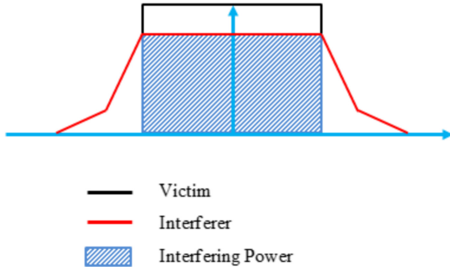
Fig. 4. Co-channel interference.
