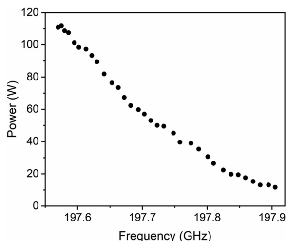
Fig. 3. Power and bandwidth of the 198 GHz gyrotron. The microwave power shown was measured at the gyrotron window. A power output of >10 W is available over 335 MHz bandwidth, with a peak power of 112 W.
