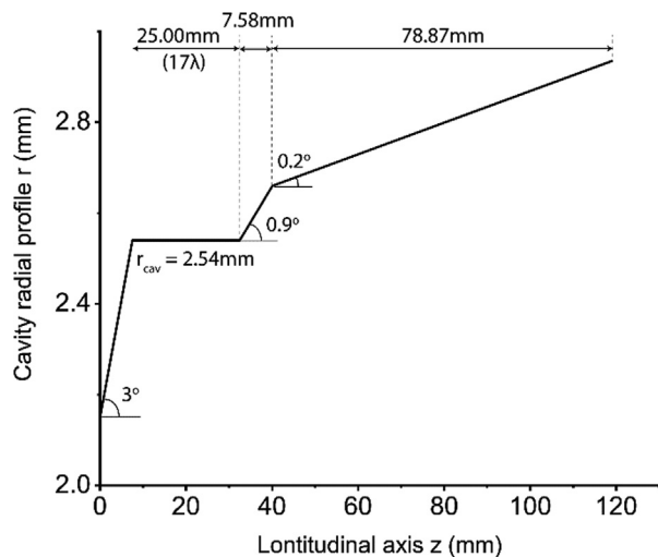
Fig. 6. Geometry of the interaction cavity and up-taper in the current 198 GHz gyrotron. The interaction cavity contains a down-taper and a 25 mm straight section. The 86 mm up-taper is machined as a separate piece.
