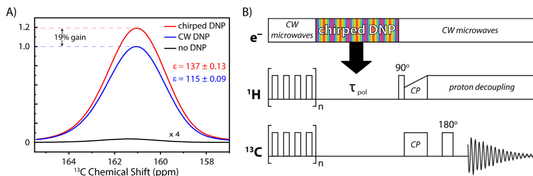
Fig. 1. (A) Spectra of 4 M [U- 15 N, 13 C] urea with 5 mM TEMTriPol-1 in d 8 -glycerol, D 2 O, and H 2 O (60%/30%/10% by volume). The black line is NMR signal without microwave irradiation. The blue line is a CW DNP-enhanced spectrum with an enhancement of 115. The red line is a DNP-enhanced spectrum using frequency chirps with an enhancement of 137. (B) The DNP cross-polarization (CP)-MAS sequence with frequency chirps (polychromatic block) used to conduct frequency-chirped DNP. See Section 2.2 for further experimental details. (For interpretation of the references to colour in this figure legend, the reader is referred to the web version of this article.)
