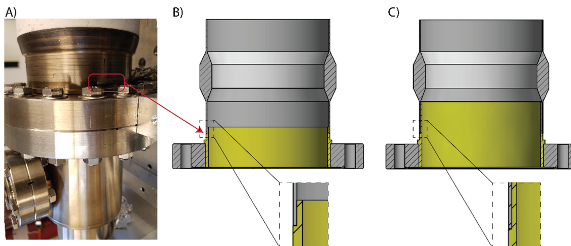
Fig. 9. Ceramic break and flange assembly. (A) Photograph of the welding on the assembly. The re-welding to fix the microleak is indicated in the red box. (B) Schematic of the assembly that had a microleak at the welding joint. The connecting part between ceramic break and flange is indicated in yellow. (C) Schematic of the improved connection between ceramic break and flange for future designs to avoid microleaks. (For interpretation of the references to colour in this figure legend, the reader is referred to the web version of this article.)
