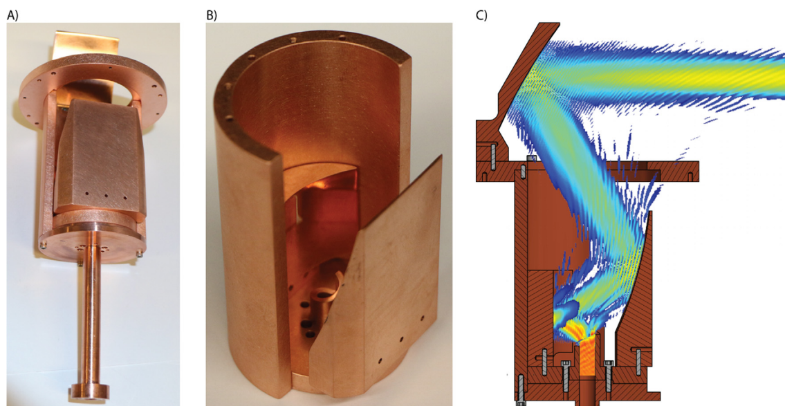
Fig. 8. Internal mode converter of the current gyrotron. (A) Photograph of the internal mode converter assembly. (B) Photograph of the lower two mirrors and the helical Vlasov launcher. (C) Section view of microwave intensity simulation in the internal mode converter. Microwave intensity plots were calculated by Bridge 12 Technologies, Inc.
