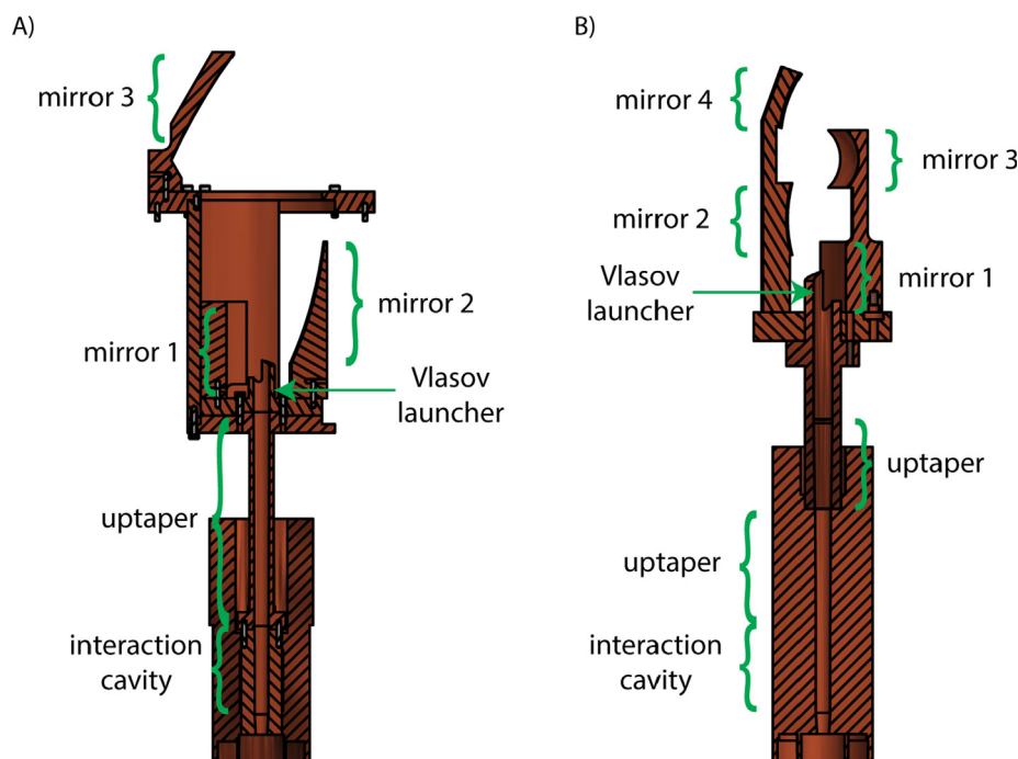
Fig. 7. Section views of internal mode converter and interaction cavity assembly of (A) the current gyrotron and (B) the Scott et al. gyrotron [43].
