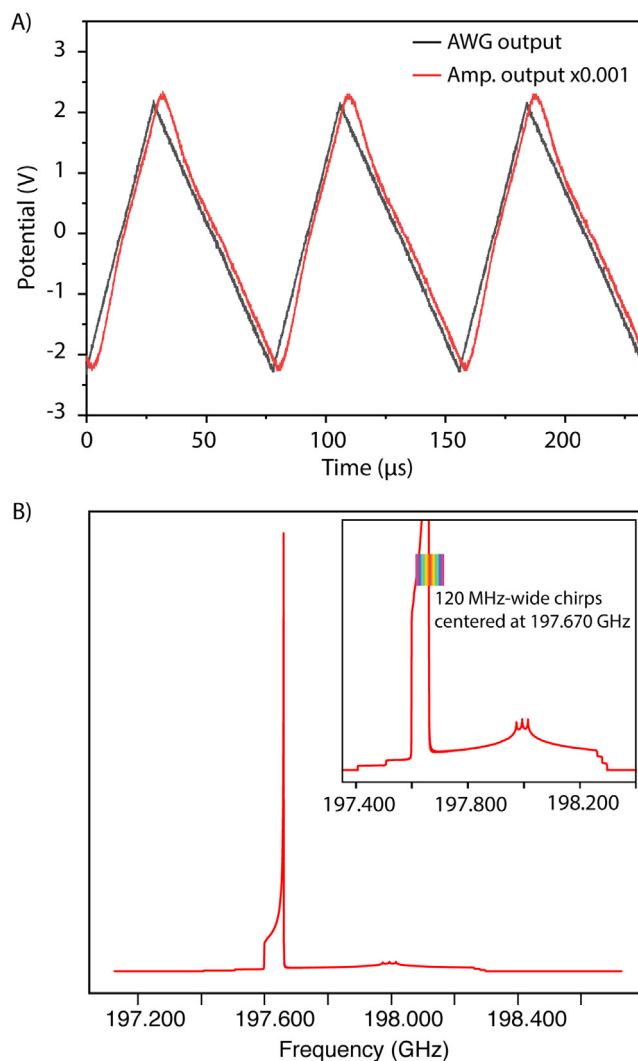
Fig. 2. (A) The voltage waveforms used for frequency-chirped DNP. The black trace is the output of the AWG and the red trace is the high-voltage amplifier output, scaled down by a factor of 1000. (B) Simulated EPR spectrum of 1:1 trityl/TEMPO combination. Both the continuous wave irradiation and frequency chirps are centered at 197.670 GHz, the condition for maximum positive cross effect enhancement [43]. The expansion on the upper-right depicts the range and location of the frequency chirps (polychromatic block) with respect to the EPR spectrum. (For interpretation of the references to colour in this figure legend, the reader is referred to the web version of this article.)
