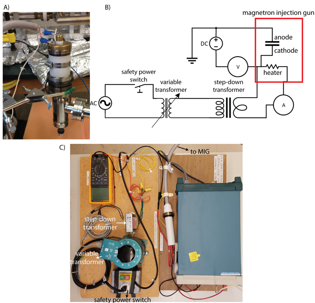
Fig. 11. MIG activation. (A) Photograph of MIG during activation. (B) Circuit diagram of the AC and DC circuits during MIG activation. (C) Photograph of the circuit diagram.
