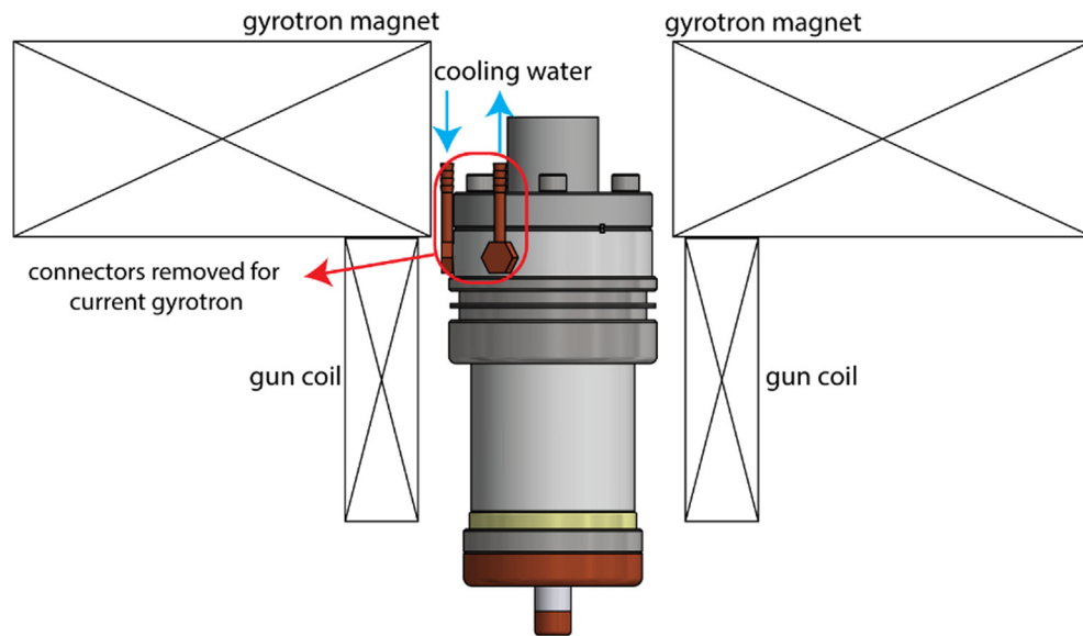
Fig. 5. Schematic of the MIG with brass connectors to water cooling lines in Scott et al. gyrotron [43]. These connectors were removed in the current gyrotron.
