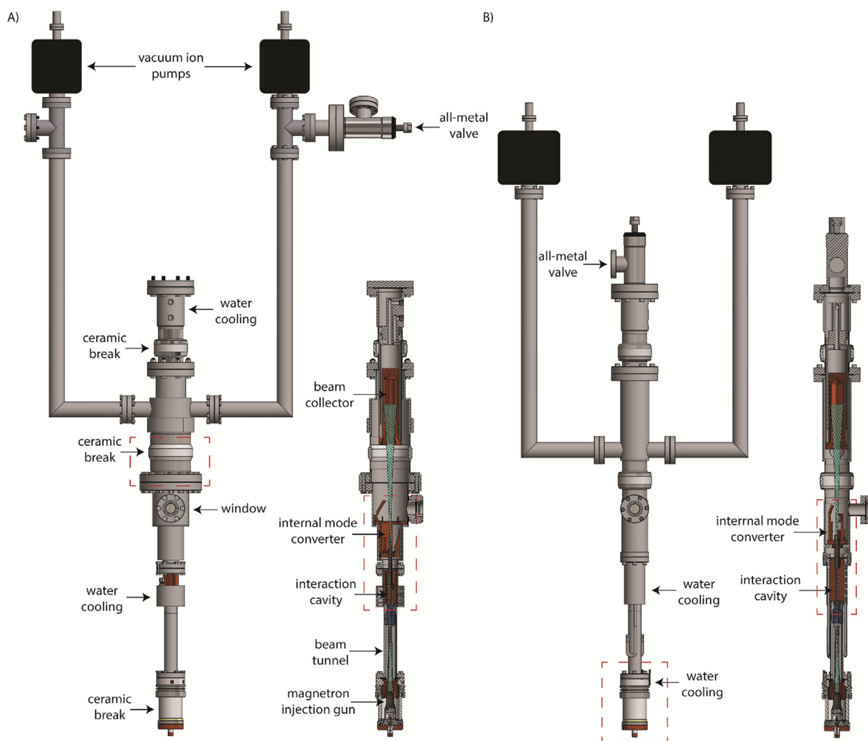
Fig. 4. Schematics of frequency-agile gyrotrons. (A) Full view and cross section of the improved gyrotron for frequency-chirped DNP experiments. (B) Full view and cross section of the gyrotron described by Scott et al. [43]. Red dashed boxes indicate areas that are shown in later figures with detail. (For interpretation of the references to colour in this figure legend, the reader is referred to the web version of this article.)
