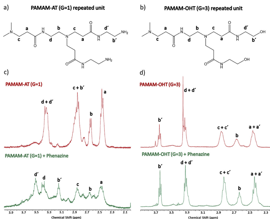
Fig. 5. Hydrogen atom labeling in the chemical structure of PAMAM-AT (G = 1) (a) and PAMAM-OHT (G = 3) (b) dendrimer. Expanded region of the ^1\text{H} NMR spectra of PAMAM-AT (G = 1) (c) and PAMAM-OHT (G = 3) (d) in absence and in presence of Phenazine, in \text{D}_2\text{O} .
