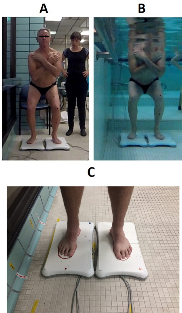
Figure 2. Testing position on land (A), in the water (B) and a close-up of foot placement on the two WBB (C). Note that in B the pool had a stepped design, with the WBB moved to the correct step height depending on the participant's height and the depth of immersion required.
