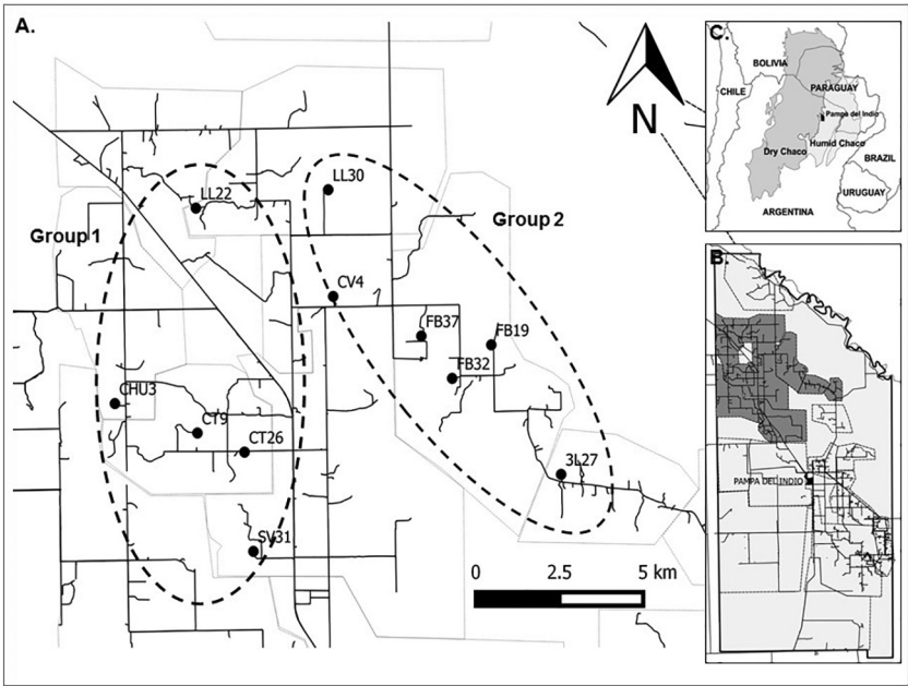
Fig. 1. Map of the study area including the location of house compounds and the two reference groups (dashed circles) previously described by Gaspe et al. (2012) in Pampa del Indio, Argentina. Western group: Group 1; eastern group: Group 2. B. Location of Area 1 (dark grey) in the Municipality of Pampa del Indio. C. Location of the Municipality of Pampa del Indio in South America.
