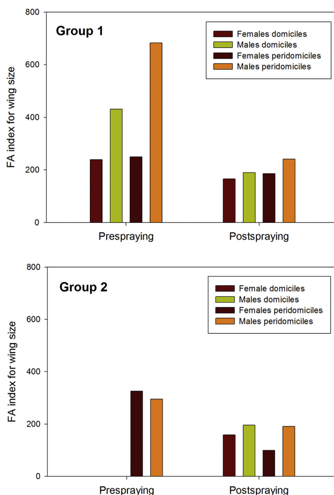
Fig. 2. Fluctuating asymmetry index for wing size for prespraying and postspraying T. infestans females and males collected in domiciles and peridomiciles from the two reference groups in Pampa del Indio, Argentina. FA indices represent the mean square (MS) of the side-individual interaction effect corrected for measurement error ( MS/ME ) as shown in the ANOVA output of Table 2.
