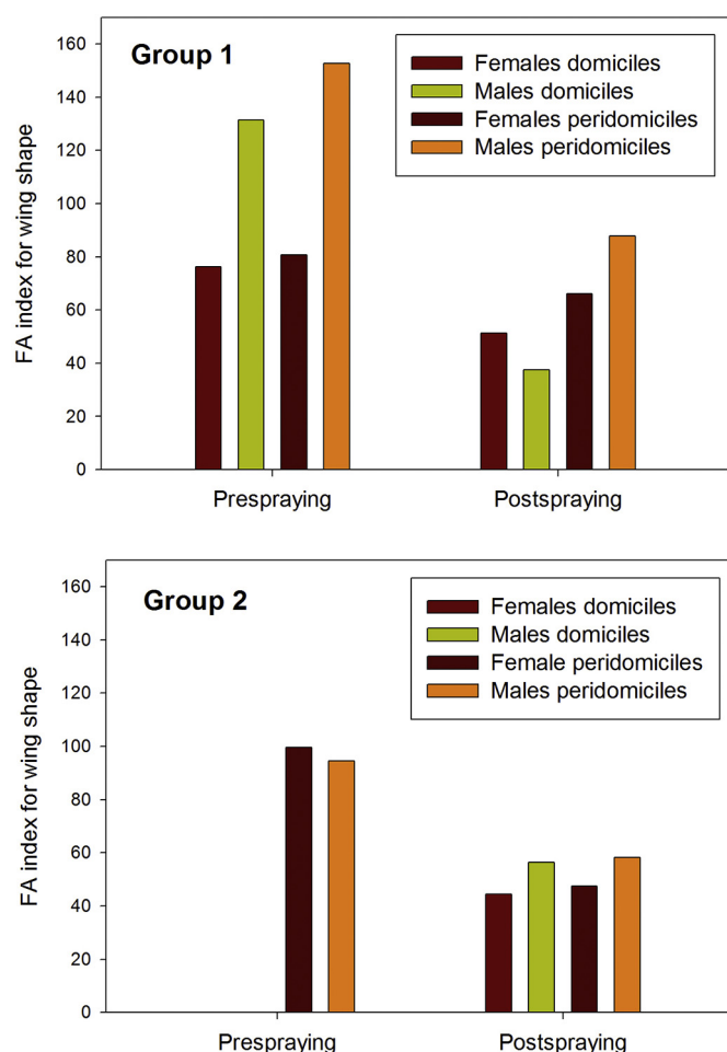
Fig. 3. Fluctuating asymmetry index for wing shape for prespraying and post-spraying T. infestans females and males collected in domiciles and peridomiciles for the two reference groups in Pampa del Indio, Argentina. FA indices represent the mean square (MS) of the side-individual interaction effect corrected for measurement error (MS/ME) as shown in the ANOVA output of Table 2.
