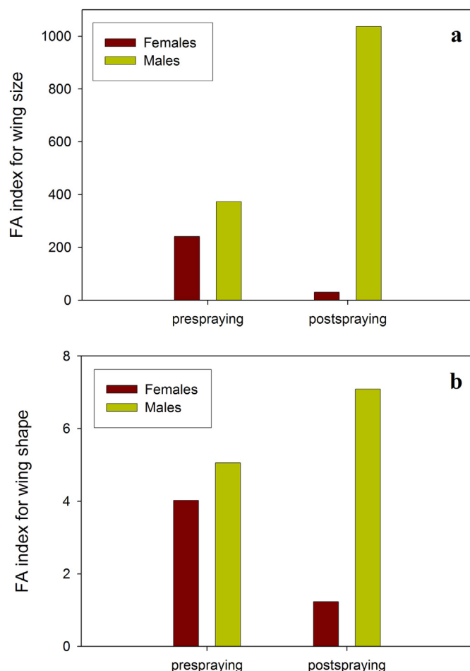
Fig. 4. Fluctuating asymmetry index for wing size and wing shape for females and males of T. infestans collected in a persistently infested peridomestic site before and after insecticide spraying in Pampa del Indio, Argentina. FA indices represent the mean square (MS) of the side-individual interaction effect corrected for measurement error (MS/ME) as shown in the ANOVA output of Table 4. a. Wing size FA indices. b. Wing shape FA indices.
