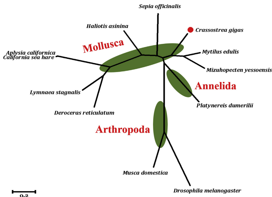
Fig. 2. Maximum likelihood (ML) phylogenetic tree based on the amino acid sequences of different FMRFamides precursor. The scale bar represented the conversion of branch length to genetic distance between clades (0.2 = 20% genetic distance). The FMRFamides used for phylogenetic analysis were from Crassostrea gigas (XP_011443786.1), Mytilus edulis (CAA10949.1), Mizuhopecten yessoensis (XP_021378855.1), California sea hare (A25790), Aplysia californica (AAA27752.1), Deroceras reticulatum (ARS01392.1), Lymnaea stagnalis (AAA63280.1), Haliothis asinine (ACD65487.1), Sepia officinalis (P91889.1), Platynereis dumerilii (AEE25641.1), Drosophila melanogaster (AAA28536.1) and Musca domestica (A6P3B2.1).
