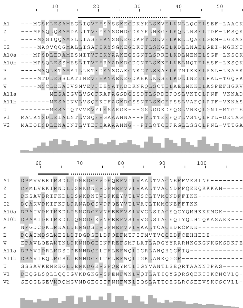
Fig. 1. Amino acid alignment of rainbow trout S100 proteins. EF-hand motifs are marked by solid (α-helices) and dotted (N-terminal S100-hand and C-terminal canonical-hand) bars. Residues with ≥50% conservation across all S100 proteins are shaded.
