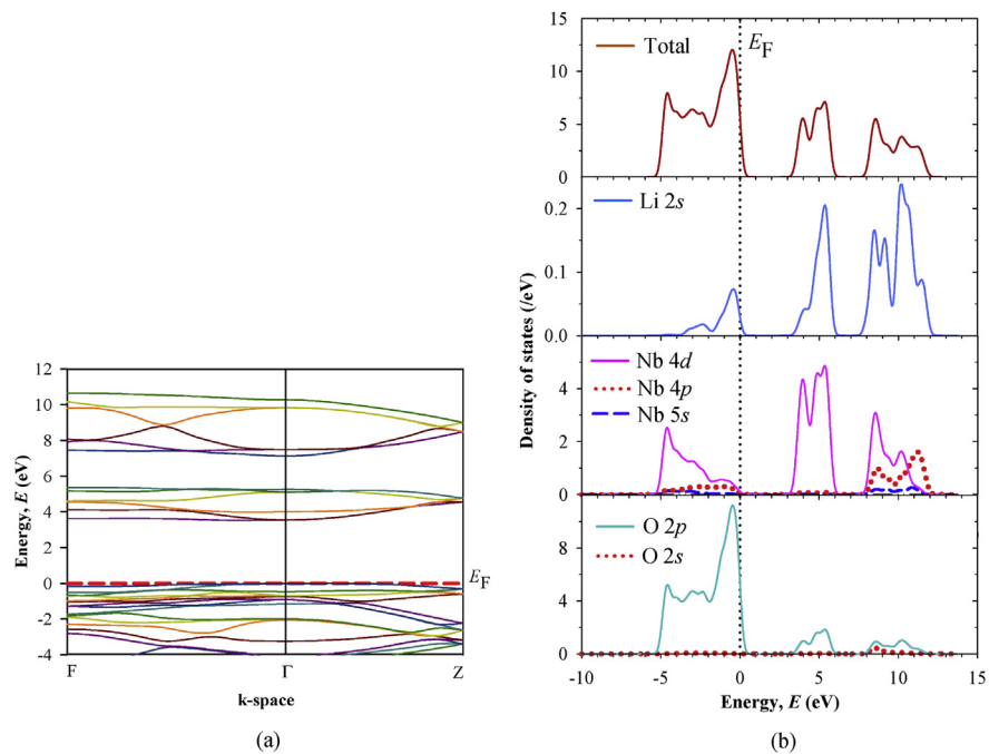
Fig. 2. (a) Electronic band structure and (b) total and partial density of states (DOS) of LiNbO 3 .
