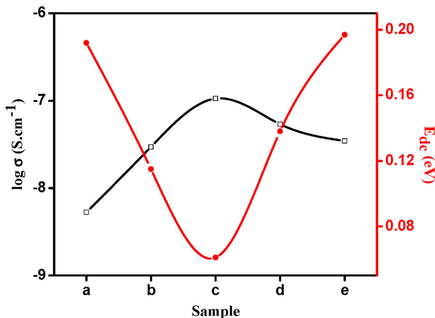
Fig. 6. Variation of \sigma_{dc} and E_{dc} for (Th-In) conducting copolymers with different stoichiometry of thiophene, indole and FeCl_3 as (a) 40:40:20, (b) 30:30:40 (c) 25:25:50 (d) 20:20:60 and (e) 10:10:80 Wt. %.
