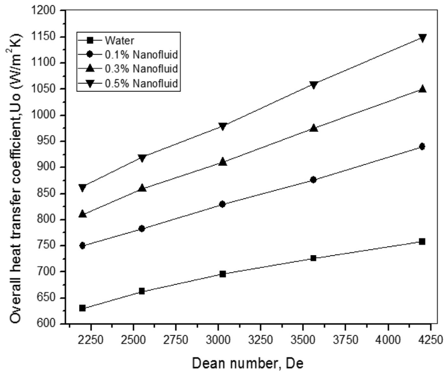
Fig. 7. Overall heat transfer coefficient Vs Dean number.
