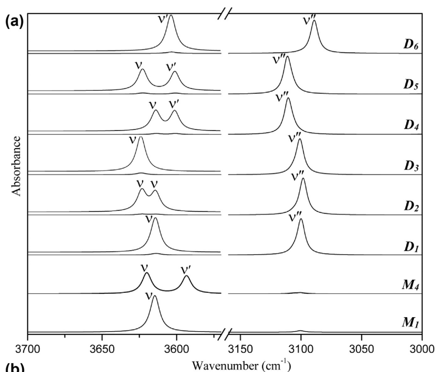
Fig. 6. (a) Computed IR spectra of monomers ( M_1 and M_4 ) and dimers ( D_1, D_2, D_3, D_4, D_5 and D_6 ) of Chelidonic acid in the 3700–3000 \text{cm}^{-1} region showing dimerization-induced characteristic band shifts and intensity enhancements. Positions of the free -\text{OH} stretching bands are marked with \nu . The positions of the intra - and inter -molecular H-bonded -\text{OH} stretching bands are marked with \nu' and \nu'' respectively. In each of the overlaid spectra in the 3700–3500 \text{cm}^{-1} , for ease of comparison, the intensities of the free ( \nu ) and H-bonded bands ( \nu' and \nu'' ) are scaled by a suitable factor. (b) Computed IR spectra of monomers ( M_1 and M_4 ) and dimers ( D_1, D_2, D_3, D_4, D_5 and D_6 ) of Chelidonic acid in the 1800–100 \text{cm}^{-1} region showing dimerization-induced characteristic band shifts and intensity enhancements. In each of the overlaid spectra in the 1000–100 \text{cm}^{-1} , for ease of comparison, the intensities of the bands are scaled by a suitable factor.
