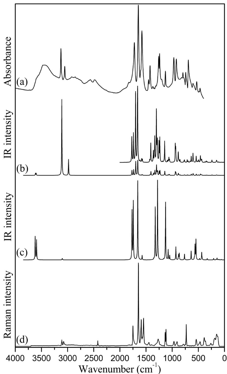
Fig. 2. Experimental FT-IR (a) and simulated IR spectra for D_4 dimer (b) and M_4 monomer (c) species of Chelidonic acid. Experimental FT-Raman spectrum (d) is also shown.
