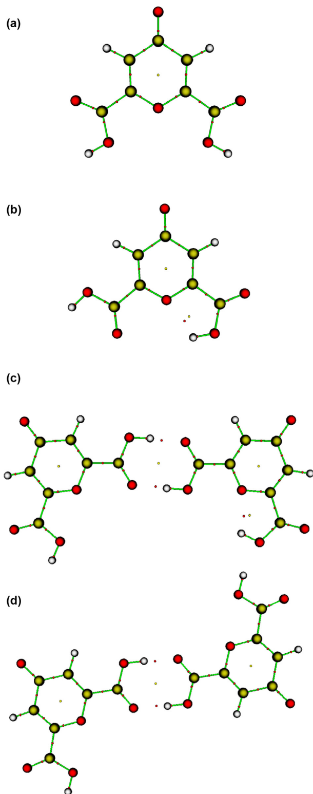
Fig. 7. Molecular structures of monomers and dimers of Chelidonic acid (Fig. 7a–7d) showing bond critical points (BCP). Topological properties of the electron density at BCP for the O...H contacts computed at B3LYP/6–311++G(d,p) level are presented in Tables 6a and 6b.
