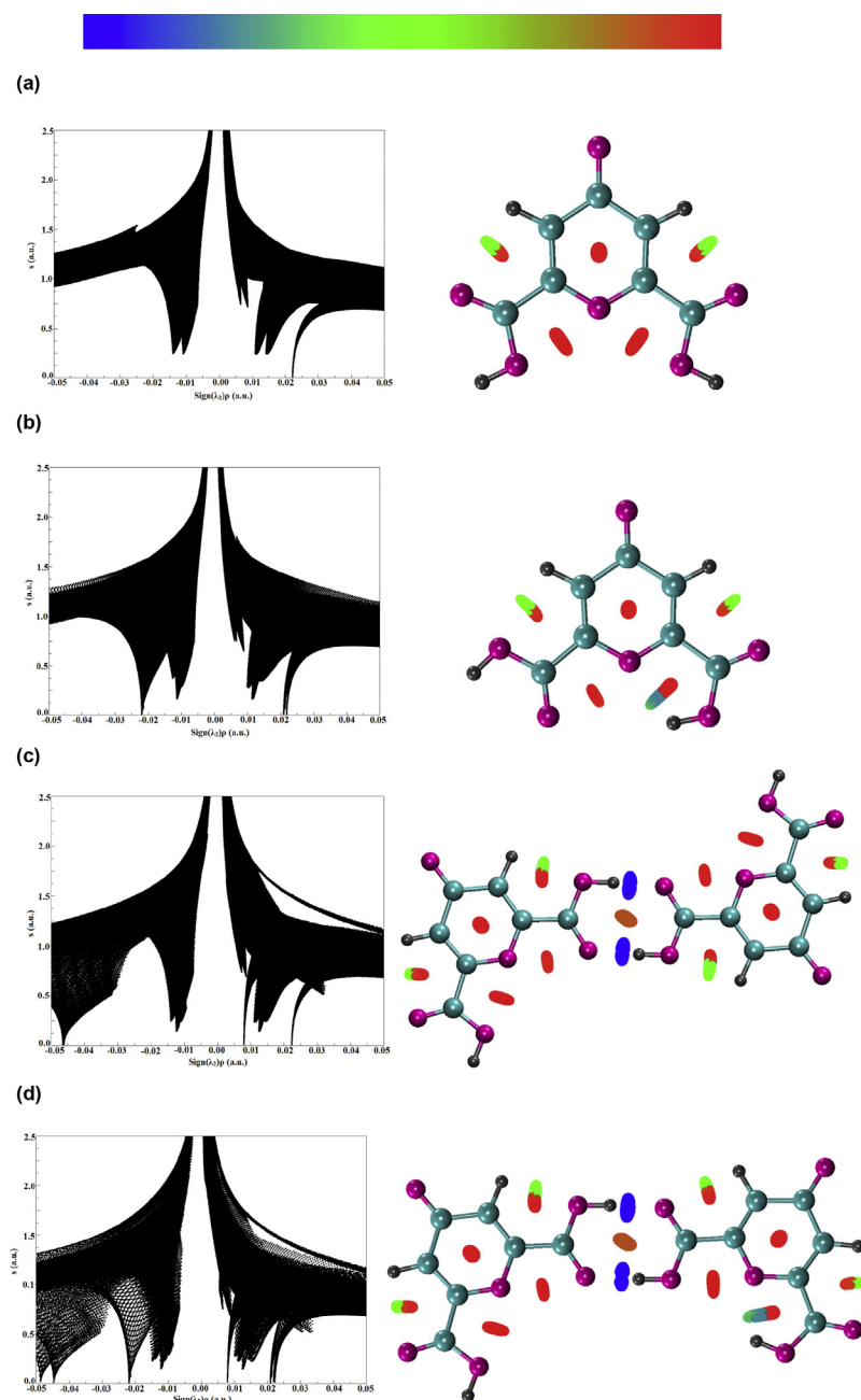
Fig. 8. Plots of the reduced density gradient, s , versus the electron density \rho(\mathbf{r}) , multiplied by the sign of second eigenvalue ( \lambda_2 ) of the electron-density Hessian matrix, \text{sign}(\lambda_2)\rho(\mathbf{r}) (left) and the corresponding isosurfaces with isovalue = 0.5 a.u (right) for Chelidonic acid structures. Isosurfaces are colored according to a BGR color scheme (Fig. 8a). Blue indicates strong attraction regime ( intra-/inter- H-bonding), green indicates weak interaction regime (such as -\text{C}-\text{H}\cdots\text{O} and van der Waals attraction), and red indicates strong repulsion regime (steric clashes). The 2D NCI plots are shown for M_1 (Fig. 8b) and M_4 (Fig. 8c) monomers and for D_1 (Fig. 8d) and D_4 (Fig. 8e) dimer structures. In each of the plots, the low-gradient spikes at about \text{sign}(\lambda_2)\rho(\mathbf{r}) = \pm 0.01 a.u represents the weak van der Waals interactions. The spikes at about \text{sign}(\lambda_2)\rho(\mathbf{r}) = -0.0219 a.u and \text{sign}(\lambda_2)\rho(\mathbf{r}) = -0.0487 a.u represents the intra- and inter- molecular H-bonds respectively.
