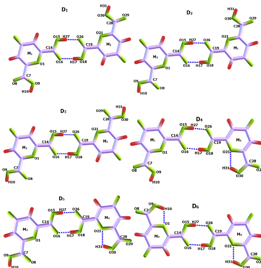
Fig. 4. Optimized structures of six dimer species of Chelidonic acid. Inter -H-bonding is in D_1 , D_2 , D_3 ; both intra - and inter -bonding is in D_4 , D_5 and D_6 .
