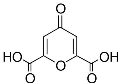
Fig. 1. Molecular structure of Chelidonic acid.
