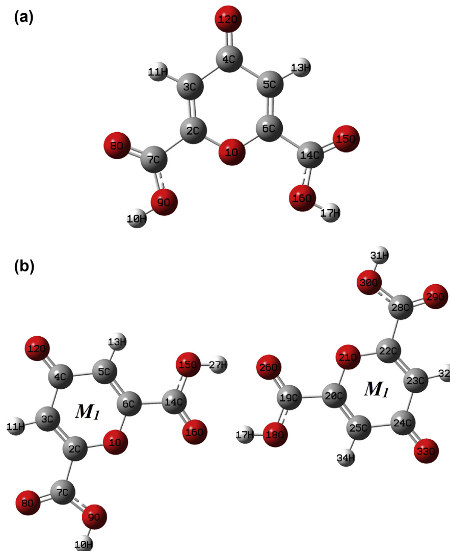
Fig. 5. Optimized structures of most stable monomer (a), and dimer (b) of Chelidonic acid.
