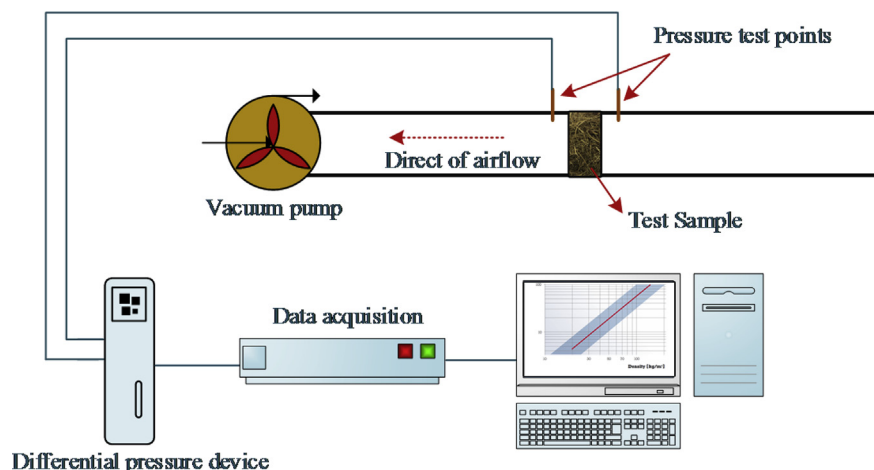
Fig. 3. Airflow resistivity measurement setup.
