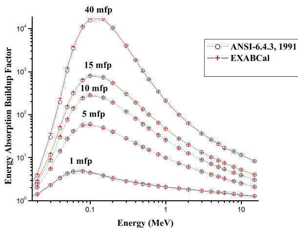
Fig. 2. Comparison of EXABCal and ANSI values of EABF of air at 1, 5, 10, 15 and 40 mfp.
