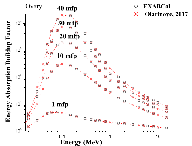
Fig. 9. Comparison of EXABCal and published values of EABF of human ovary at 1, 10, 20, 30 and 40 mfp.
