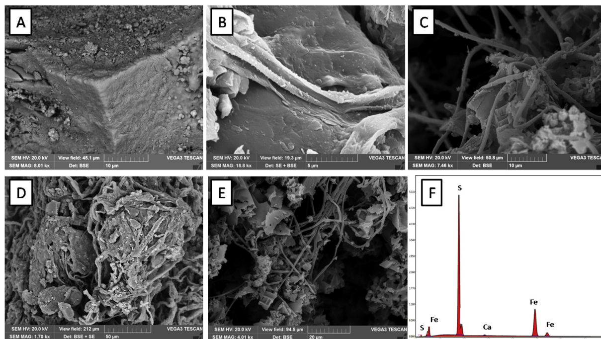
Fig. 1. A) ESEM image of unaltered pyrite crystal without evidence of mycological biofilm and hyphae. B) Detail of a pyrite crystal surface with evidences of bioweathering represented by pitting, etching and dissolution channel placed in correspondence of T. terrestris hyphae. C) ESEM image showing altered pyrite crystal completely enveloped by T. terrestris hyphae. D) Detail of T. terrestris hyphae enveloping pyrite crystal. E) ESEM image evidencing the high degree of colonization by T. terrestris mycelium with interstitial idiomorphic pyrite crystals, lamellar calcium-sulphate (presumably gypsum) and microcrystalline aggregates of Fe-oxyhydroxides. F) EDS spectra of the area reported in Fig. E.
