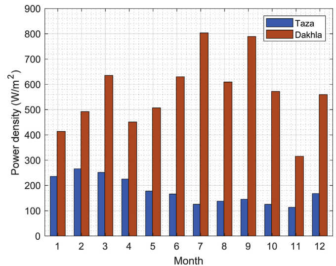
Fig. 8. Monthly wind power density from Weibull distribution of Dakhla and Taza sites at 100 m height.
