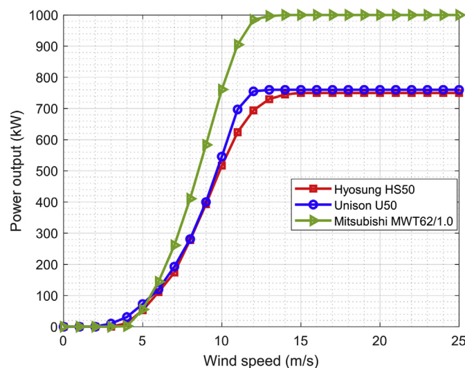
Fig. 9. Power curves of three turbines for a hub height of 50 m.
