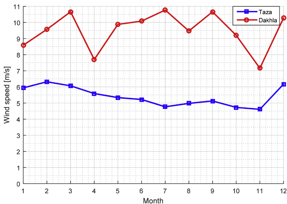
Fig. 2. Monthly mean wind speed at the height 100 m.
