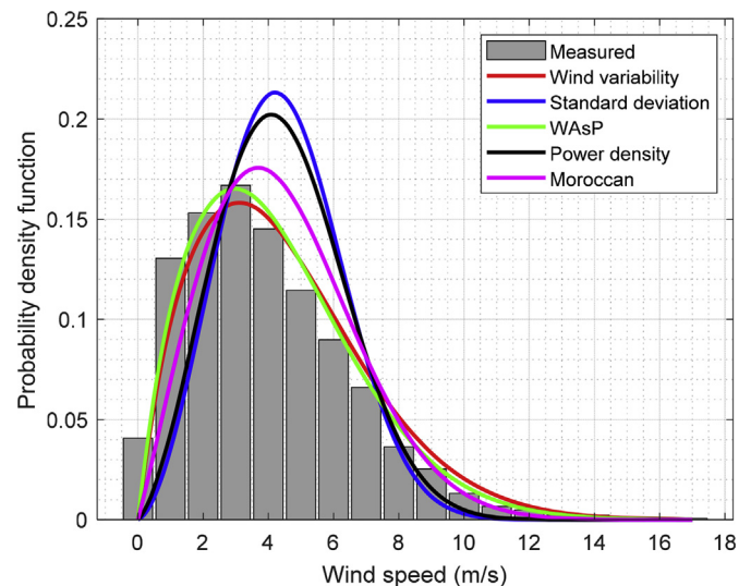
Fig. 4. Comparison of the frequency calculated by the four methods for Taza site.
