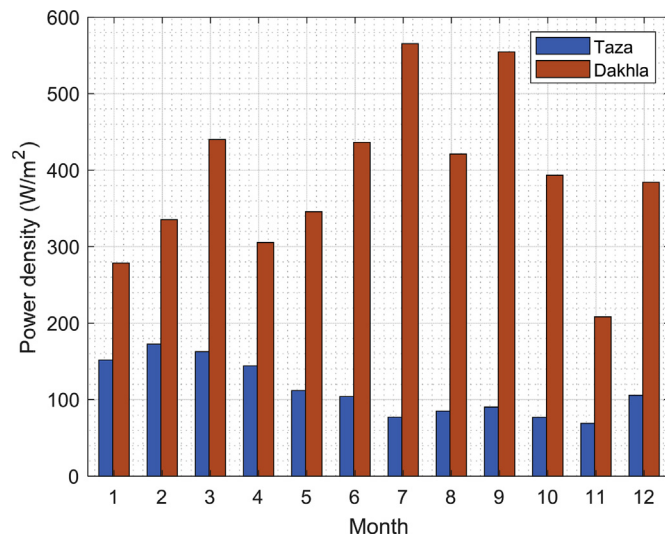
Fig. 7. Monthly wind power density from Weibull distribution of Dakhla and Taza sites at 50 m height.
