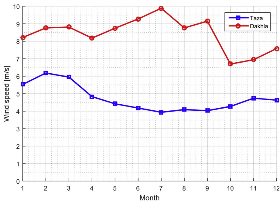
Fig. 1. Monthly mean wind speed at the height 50 m.
