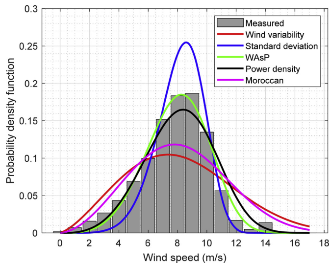
Fig. 3. Comparison of the frequency calculated by the four methods for Dakhla site.
