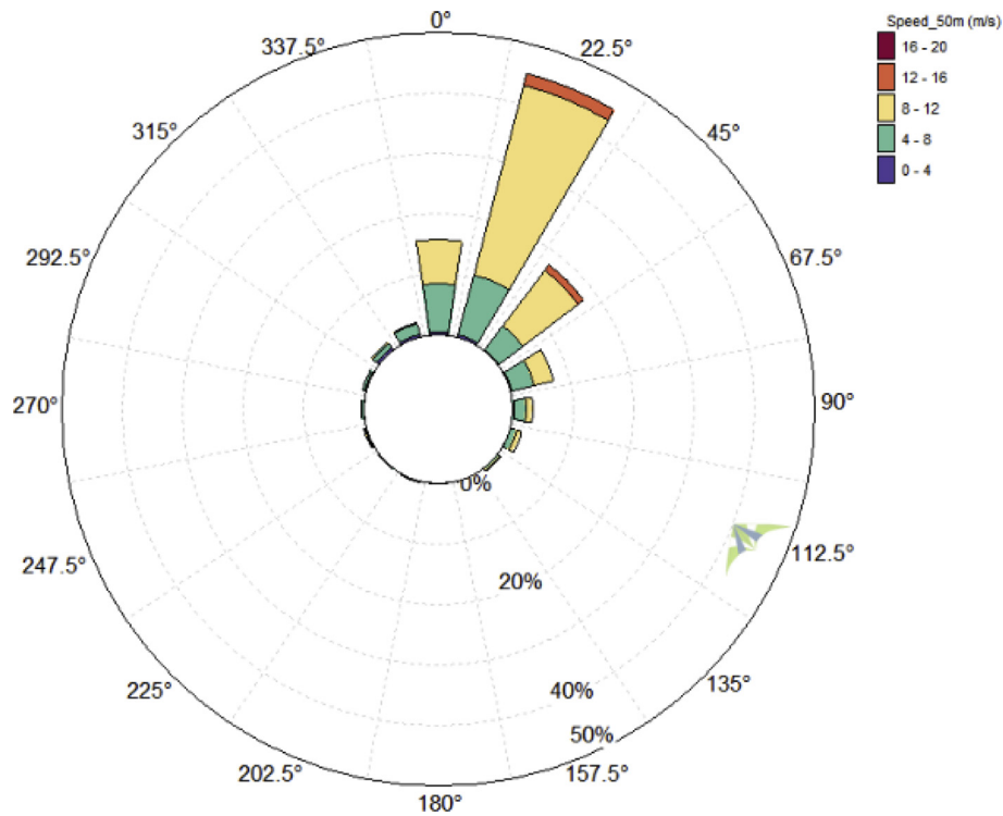
Fig. 6. Wind rose polar diagram for Dakhla site.
