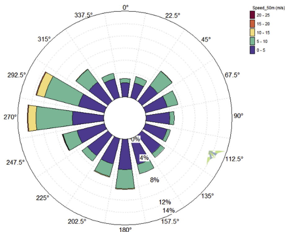
Fig. 5. Wind rose polar diagram for Taza site.
