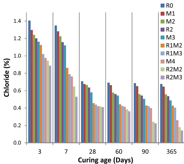
Fig. 9. Graph showing the percentage of chloride ion at 10–20 mm depth w.r.t Days of curing in water.
