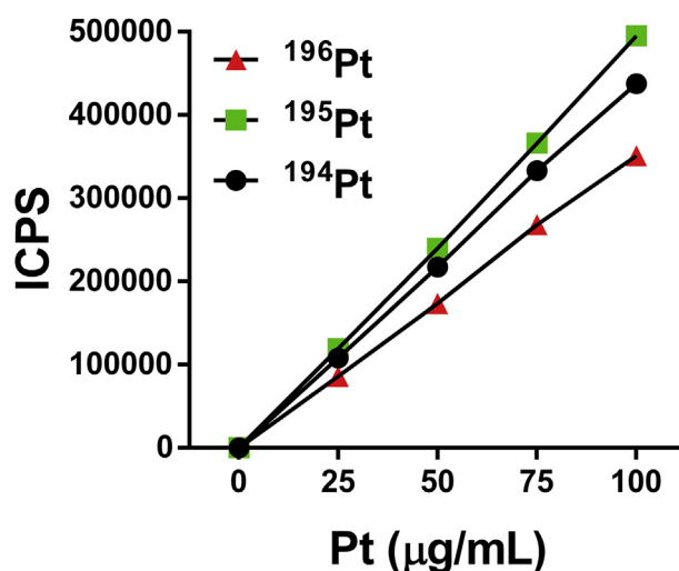
Fig. 1. Calibration graph and the best line equation for ^{194}\text{Pt} , ^{195}\text{Pt} and ^{196}\text{Pt} isotopes by ICP-MS.
