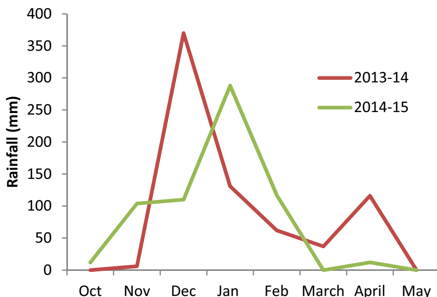
Fig. 1. Monthly rainfall totals at Masomera Village, Marondera district, Zimbabwe, in the 2013/14 and 2014/15 seasons.
