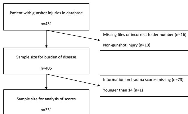
Fig. 1. Flow diagram of study sample
