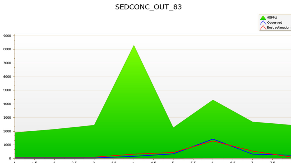
Fig. 2. Sub-basin 83 comparison of simulated and observed sediment during the calibration period (March–October 2018).
