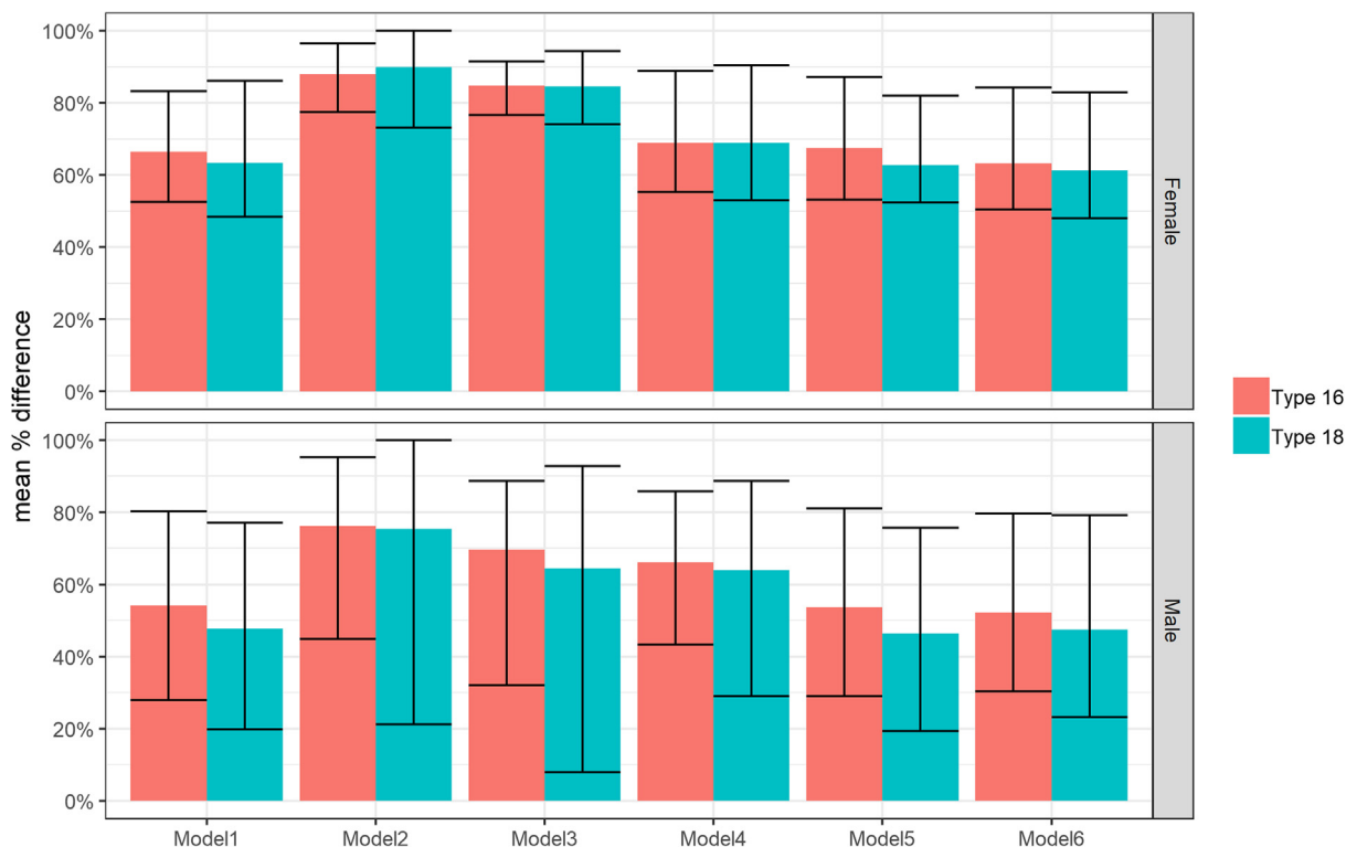
Fig. 2. Mean percentage reduction in HPV16/18 prevalence in 2045 for individuals aged 15+ with prophylactic vaccine efficacy of 100%. Vaccination coverage of 9 year olds girls is assumed constant between 2014 and 2045 at 90%.
