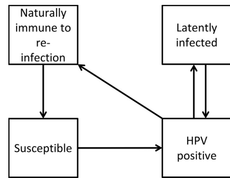
Fig. 1. Natural history of human papillomavirus in Model 1.
