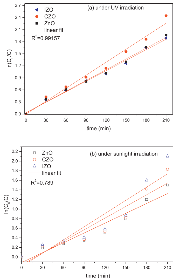
Fig. 8. Plot of \ln\left(\frac{C_0}{C}\right) versus irradiation time for ZnO, CZO and IZO thin films, under (a) UV and (b) sunlight irradiation.
