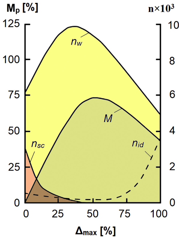
Fig. 12. Dependence of the rate M_p and the number of pulses n on the discharge gap \Delta [74].
