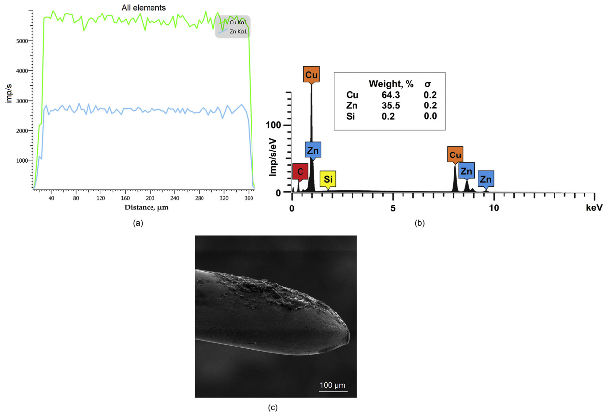
Fig. 14. Characterization of wire tool after WEDM of the sample made of VOK-6O conductive ceramic composite: (a) distribution of all chemical elements along the diameter; (b) X-ray spectrometry analysis; (c) SEM of the wire tool break point with the presence of the erosion traces.
