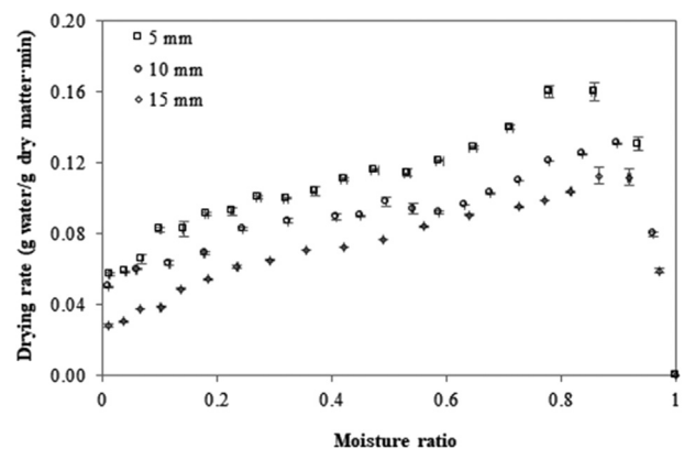
Fig. 6. DR curves of VIR drying of CQ of different material thicknesses.
