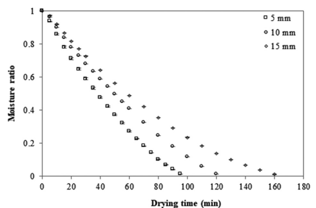
Fig. 5. MR curves of VIR drying of CQ of different material thicknesses.
