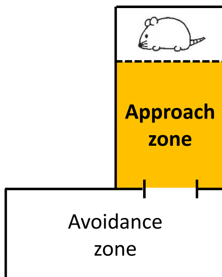
Fig. 1. Apparatuses for the social preference and the social approach tests. (a) The apparatus for the social preference test was composed of a neutral area and two zones (object and animal). A test animal can enter the object or the animal zone from the neutral area. Each zone contains a small chamber separated by a clear punch-out board. An object (rubber frog) and a stimulus animal were put in the object and animal chambers, respectively. (b) The apparatus for the social approach test was composed of avoidance and approach zones. The approach zone contained a small chamber separated by a clear punch-out board. A stimulus animal was put in the chamber of the approach zone.
