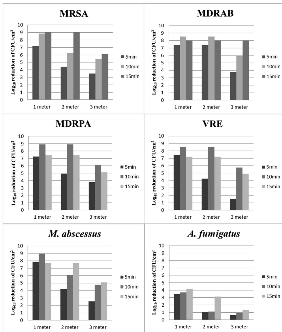
Figure 2. The effectiveness of the Hyper Light P3 device on reducing various strains of bacteria or fungi expressed in \text{log}_{10} reduction of CFU/cm 2 . Abbreviations: CFU, colony-forming units; MRSA, methicillin-resistant Staphylococcus aureus ; MDRAB, multidrug-resistant Acinetobacter baumannii ; MDRPA, multidrug-resistant Pseudomonas aeruginosa (MDRPA); VRE, vancomycin-resistant Enterococcus faecium ; M. abscessus , Mycobacterium abscessus ; A. fumigatus , Aspergillus fumigatus
