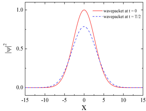
Figure 2. The wavepacket’s profiles at t = 0 and t = T/2 in the toy model (19), with the initial wavepacket assuming the Gaussian form (15). The width of the initial wavepacket is set 5.46 in units of \hbar/k .
