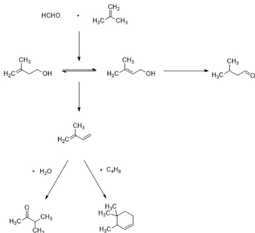
Fig. 4. Reaction network.
