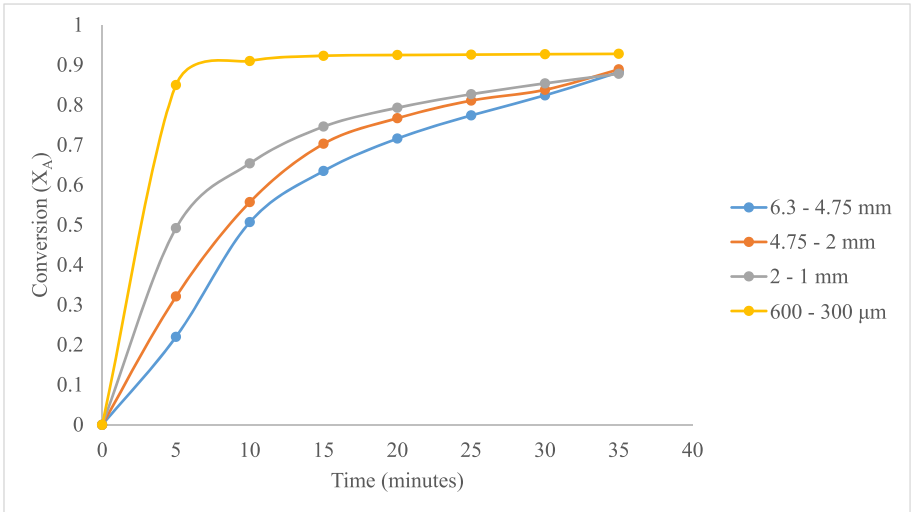
Fig. 3. Effect of 1.2M acetic acid treatment on \text{Ca}^{2+} conversion ( X_A ) in snail shell demineralization.
