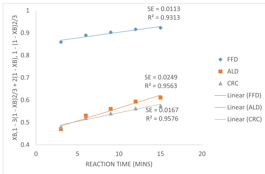
Fig. 7. SCM for 600–300 \mu\text{m} snail shell particle sizes demineralization using 1.2M acetic acid.
