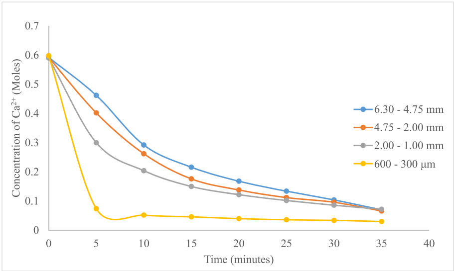
Fig. 2. Effect of 1.2M acetic acid treatment on \text{Ca}^{2+} concentration on snail shell demineralization.
