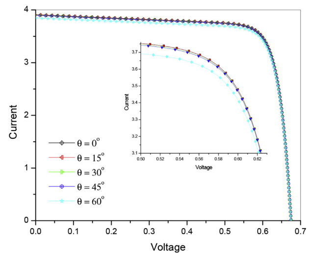
Fig. 6. Current – voltage characteristics of silicon solar cell at various angles of incidence.
