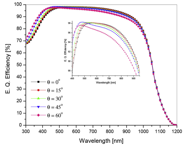
Fig. 5. Variation of external quantum efficiency as a function of wavelength at different angles of incidence.
