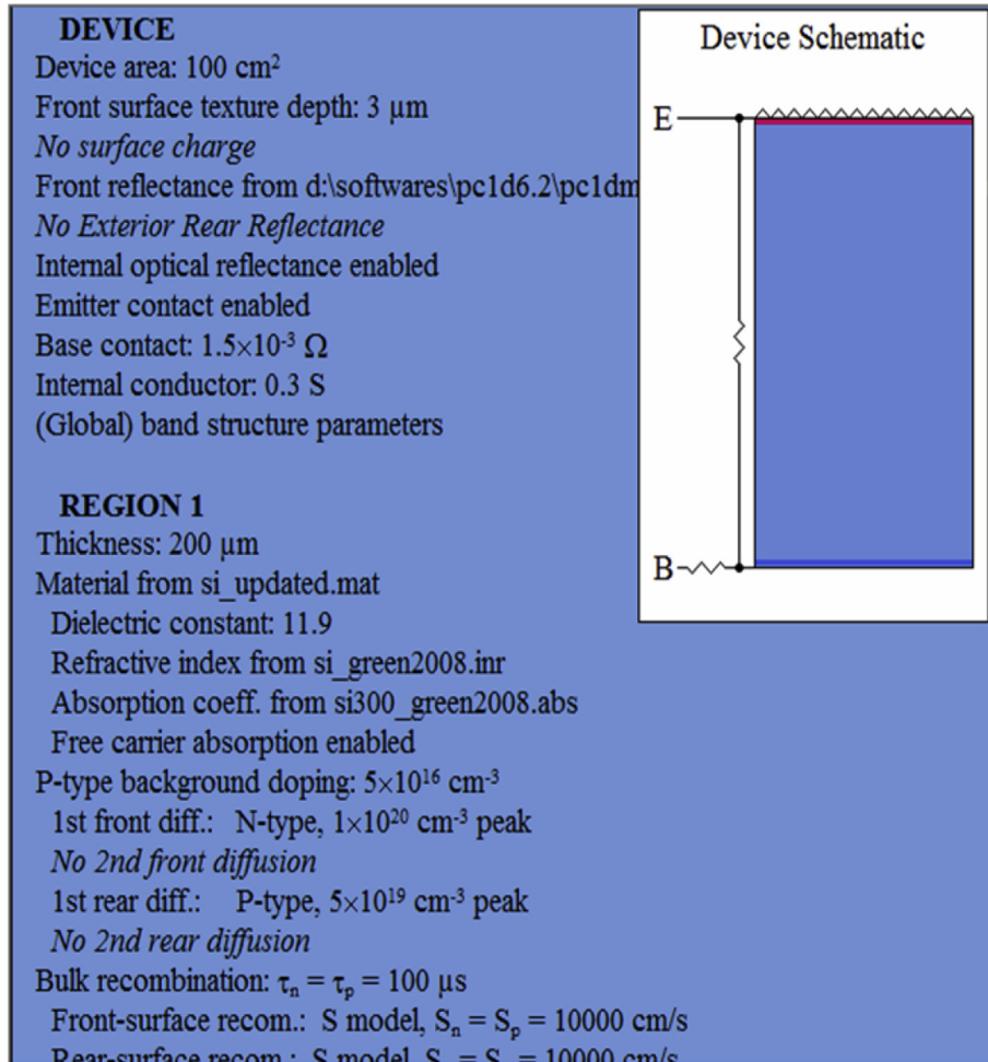
Fig. 2. Summary of simulation parameters for PC1Dmod Model.
