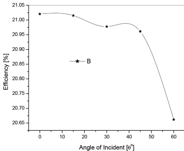
Fig. 7. Variation of conversion efficiency of silicon solar cell as a function of angle of incidence of sunlight.
