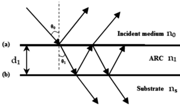
Fig. 1. Reflection at interface between two media.
