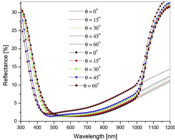
Fig. 4. Reflectance spectra as a function of wavelength for various angles of incidence. Solid lined for numerically calculated (using TMM) and line plus symbol obtained from PC1D.
