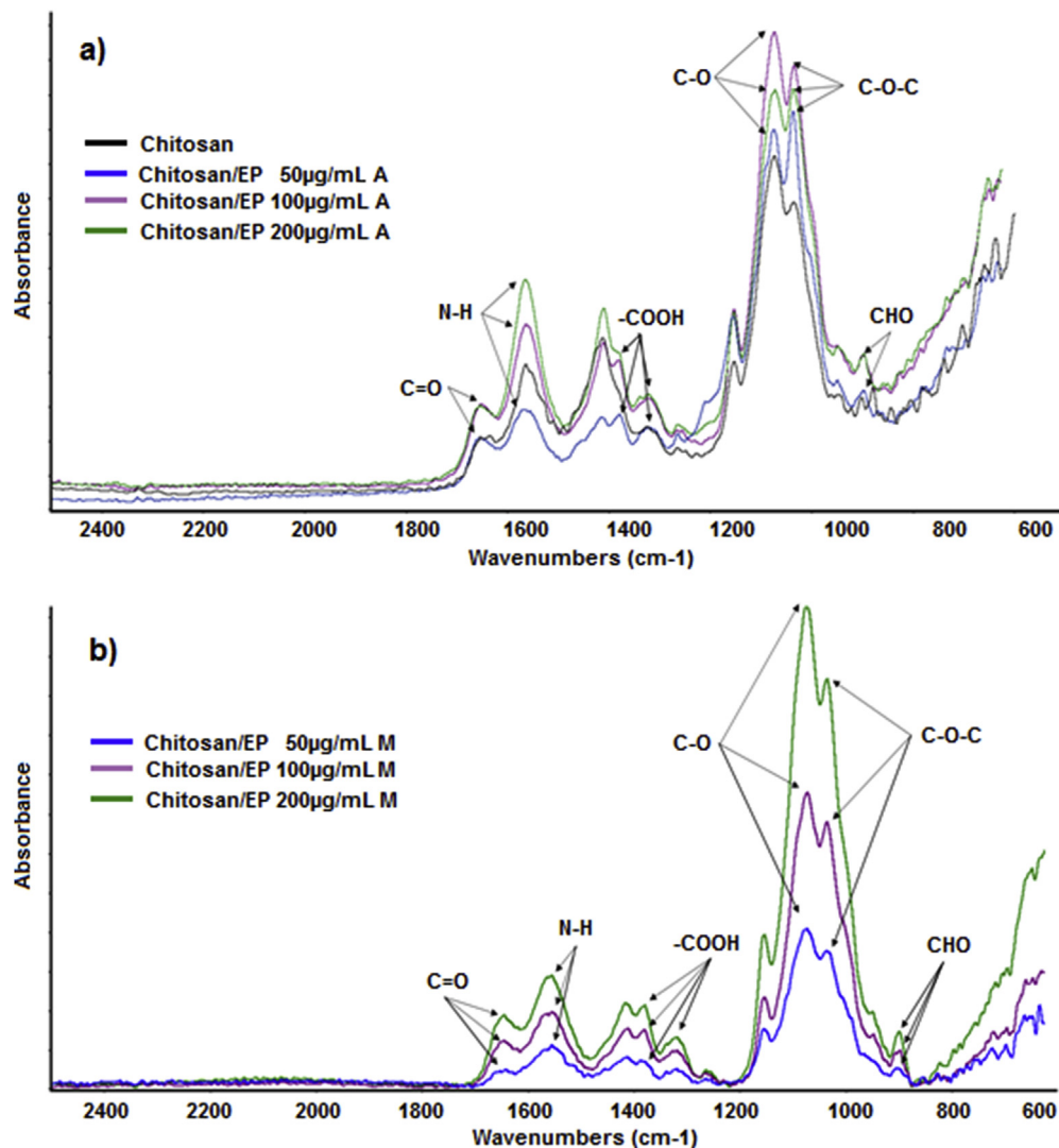
Fig. 2. Infrared spectra of the scaffolds: a) chitosan, chitosan/EP 50 \mu\text{g/mL} A, chitosan/EP 100 \mu\text{g/mL} A, chitosan/EP 200 \mu\text{g/mL} A, b) chitosan EP 50 \mu\text{g/mL} M, chitosan/EP 100 \mu\text{g/mL} M, chitosan/EP 200 \mu\text{g/mL} M.
