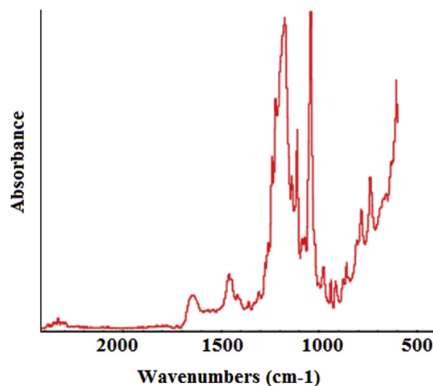
Fig. 1. Infrared spectrum of the pure EP protein.
