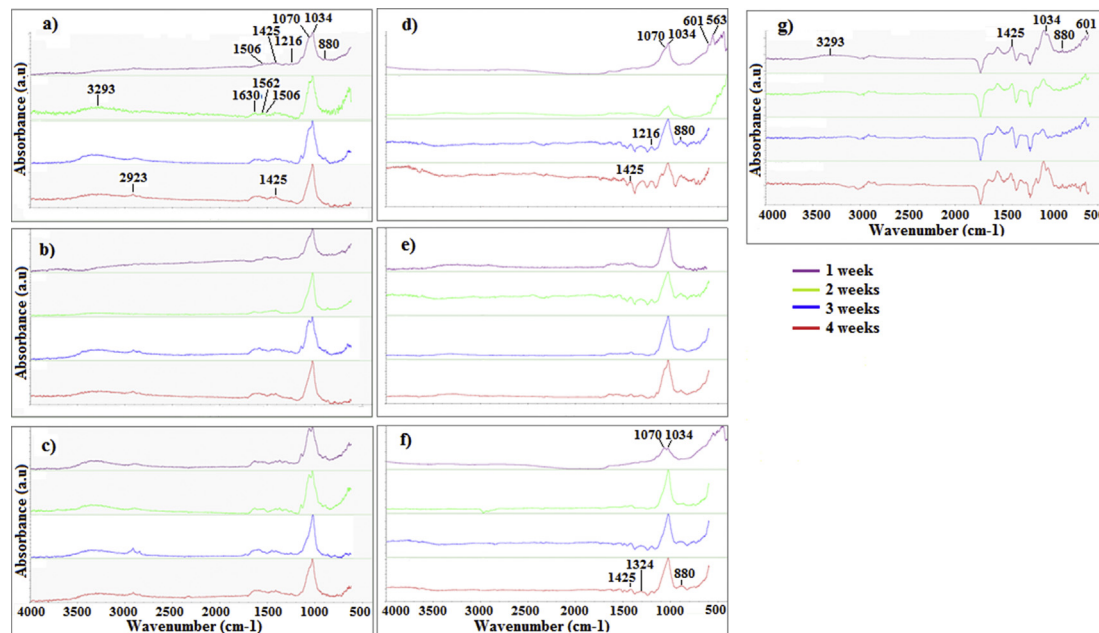
Fig. 3. Infrared spectra of the scaffolds after 4 weeks exposure to the SBF 1.5X solution. Chitosan spectrum (without exposure) was subtracted from: a) scaffold of chitosan/EP 50 µg/mL A and b) scaffold of chitosan/EP 50 µg/mL M; c) scaffold of chitosan/EP 100 µg/mL A and d) scaffold of chitosan/EP 100 µg/mL M; e) scaffold of chitosan/EP 200 µg/mL A and f) scaffold of chitosan/EP 200 µg/mL M, and g) scaffold of chitosan.
