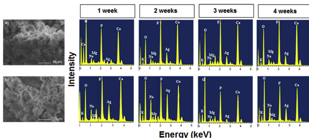
Fig. 6. Images of SEM and EDS spectrum of the apatite layer formed on the scaffolds of a) chitosan/EP 50 µg/mL A y b) chitosan/EP 100 µg/mL M after soaking in SBF.
