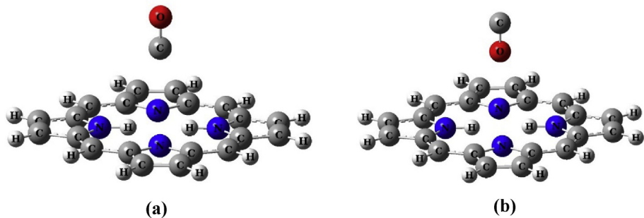
Fig. 2. The optimized structures for CO/P complex, calculated at B3LYP/LanL2DZ. (a) mode 1, and (b) mode 2.
