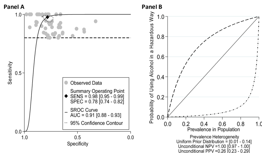
Fig. 2. Panel A: Aggregated ROC curve for n = 53 studies (grey circles) of screening instruments reporting diagnostic accuracy data; dashed horizontal line presenting the sensitivity inclusion criterion ( \geq .80 ). Panel B: Probability of using alcohol in a hazardous way depending on prevalence for positive (long dashed) and negative (short dashed) test results.
