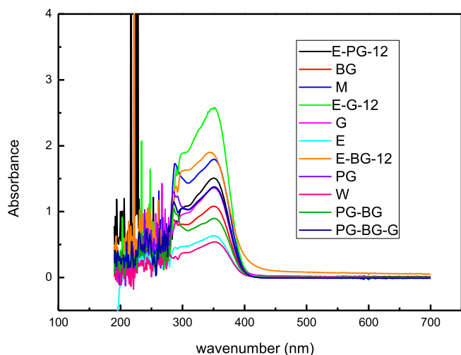
Fig. 3. UV-Vis absorbance spectrum of C. oleifera Abel dregs extracts at room temperature extracted and at 100x dilution.
