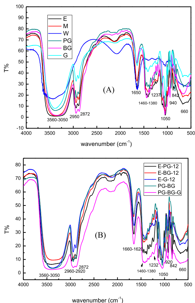
Fig. 2. FTIR spectrums of C. oleifera Abel dregs extracts. (A) Extract by single solvents at room temperature, and (B) extract by mixed solvents at room temperature.
