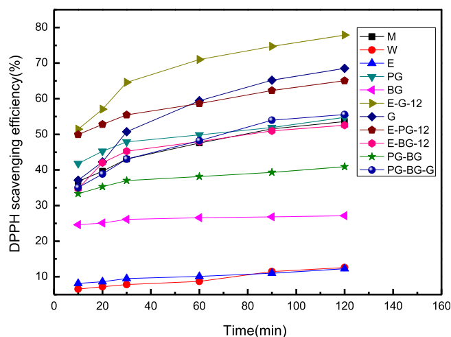
Fig. 4. DPPH scavenging efficiency of C. oleifera Abel dregs extracts at microwave-heating extracted.
