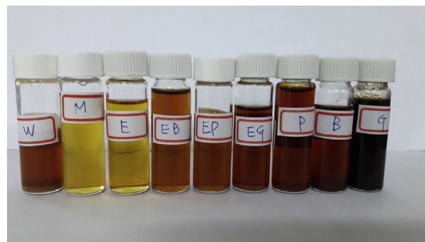
Fig. 1. Filtrates of C. oleifera Abel dregs extract by microwave-heated.
