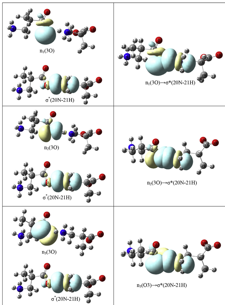
Fig. 7. Electron density maps of selected NBOs involved in \text{N-H}\cdots\text{O} bonding in D_1 . Donor (lone pair orbital of 3O) and acceptor (antibonding orbital of 20N–21H) NBOs are shown separately in left columns and their overlapping due to H-bonding is shown in right columns. Green and yellow colours of the orbitals correspond to positive and negative signs respectively.
