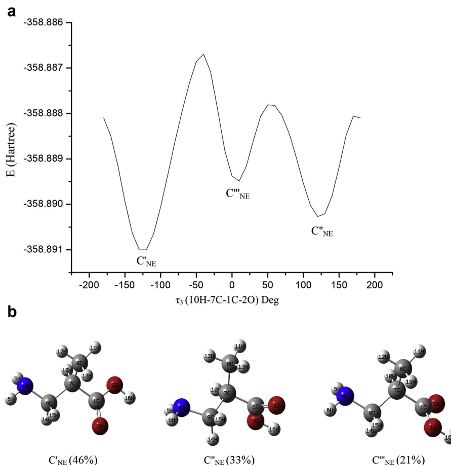
Fig. 3. (a). PES curve for the dihedral angle \tau_3 = 10\text{H}-7\text{C}-1\text{C}-2\text{O} yielding the stable conformers \text{C}'_{\text{NE}} , \text{C}''_{\text{NE}} and \text{C}'''_{\text{NE}} of DL-3-Aminoisobutyric acid at RHF/3-21G level. (b). Optimized structures ( \text{C}'_{\text{NE}} , \text{C}''_{\text{NE}} and \text{C}'''_{\text{NE}} ) of DL-3-Aminoisobutyric acid in NE form at B3LYP/6-311++G(d, p) level (values given in paranthesis are their Boltzmann populations).
