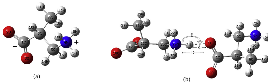
Fig. 4. Optimized (a) C_{2v} , (b) D_1 structures of DL-3-Aminoisobutyric acid showing the hydrogen bonding parameters d , D , \theta (parameter values are given in Table 2).
