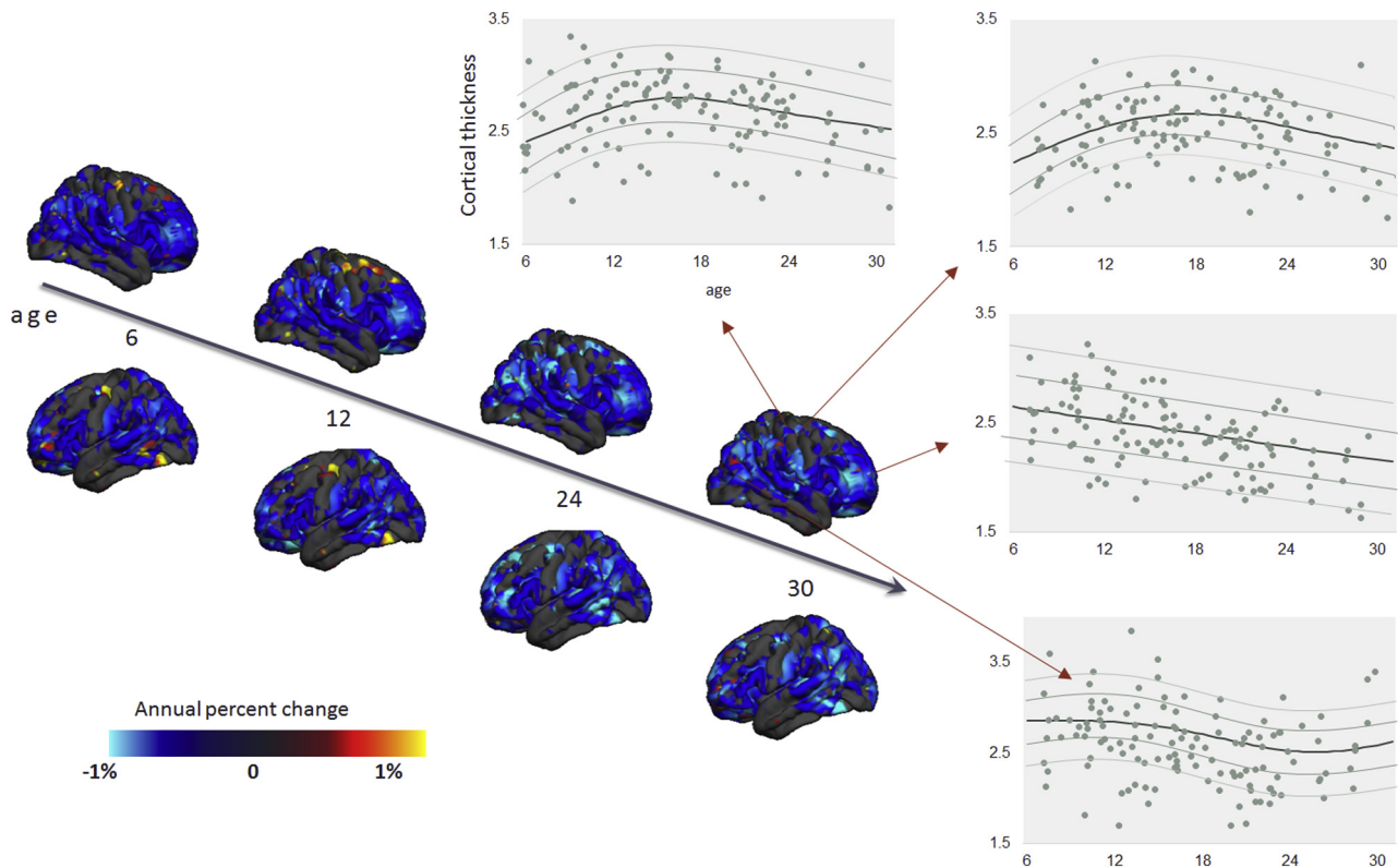
Figure 2. Normative model of developmental changes of cortical thickness across the developmental range in the typically developing male cohort (the model was estimated using both genders). Cortical thickness was predicted using a trained normative model across the age range of 6 to 31 years of age. The predicted cortical thickness map was thresholded so that only vertices that could accurately predict the true cortical thickness in the healthy cohort under cross-validation were retained (Pearson correlation, p < .05 , false discovery rate). Blue and yellow vertices indicate reduced and increased cortical thickness, respectively. Moreover, the predicted cross-sectional developmental trajectories of cortical thickness in four randomly selected vertices are shown.
