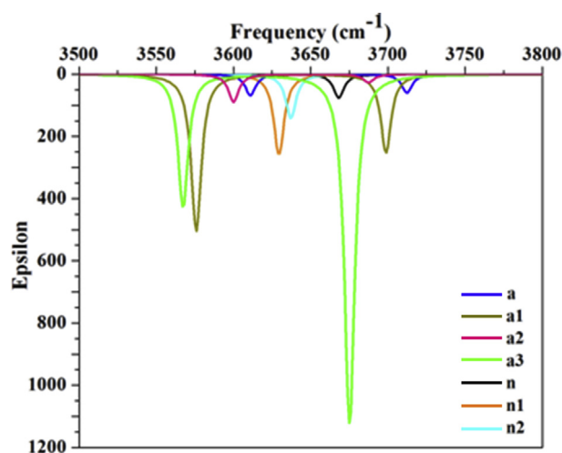
Fig. 3. Infrared spectra in the 3500–3800 \text{cm}^{-1} spectral range of isolated monomers ( a and n ) and their hydrogen bonded complexes ( a1 , a2 , a3 , n1 , n2 ) computed with the \omega B97XD/6-311++G (d,p) method.
