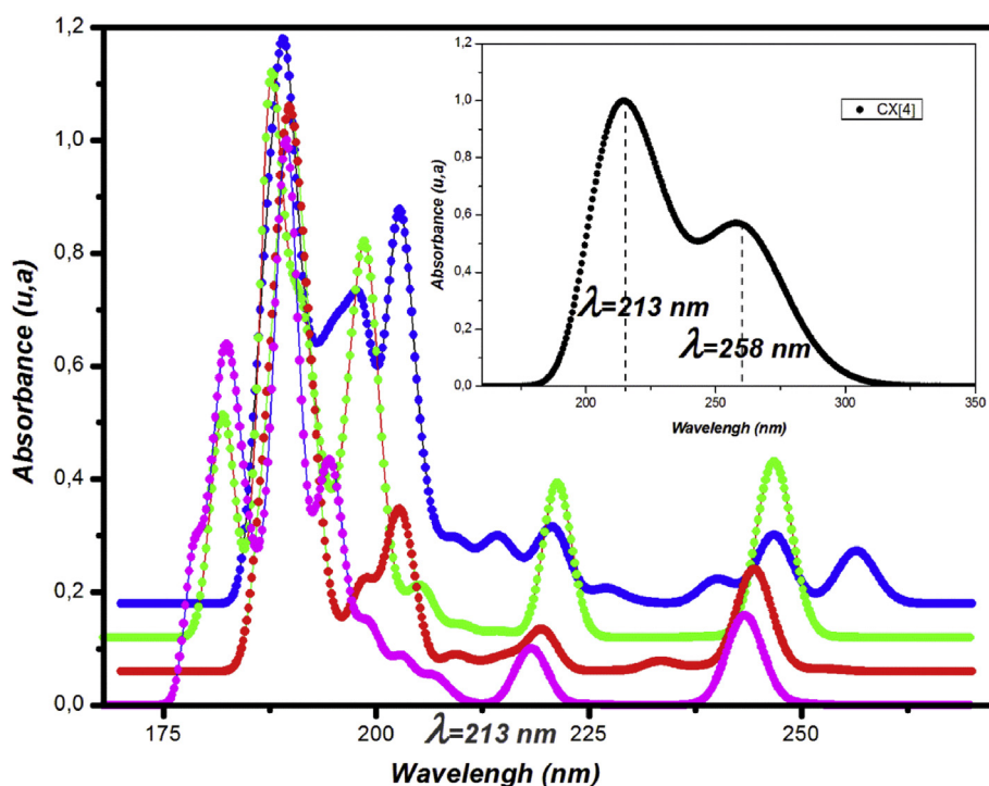
Fig. 2. Absorption spectrum of capture of TFSI - ion by calix[4]arene molecule (Blue: CX[4]-TFSI - 4, Green: CX[4]-TFSI - 2, Red: CX[4]-TFSI - 1, Magenta: CX[4]-TFSI - 3) (according to the order of stability).
