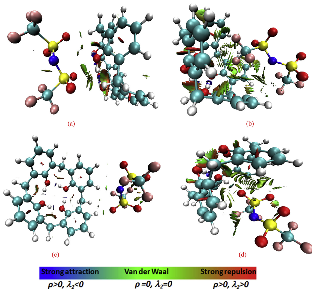
Fig. 4. NCI isosurfaces for the inclusion complexes CX[4]-TFSI - 1 (a), CX[4]-TFSI - 2 (b), CX[4]-TFSI - 3 (c) and CX[4]-TFSI - 4 (d). The iso-surfaces were constructed with RGD = 0.5 au and the blue-red colors scaling from -0.01 to 0.01 au.
