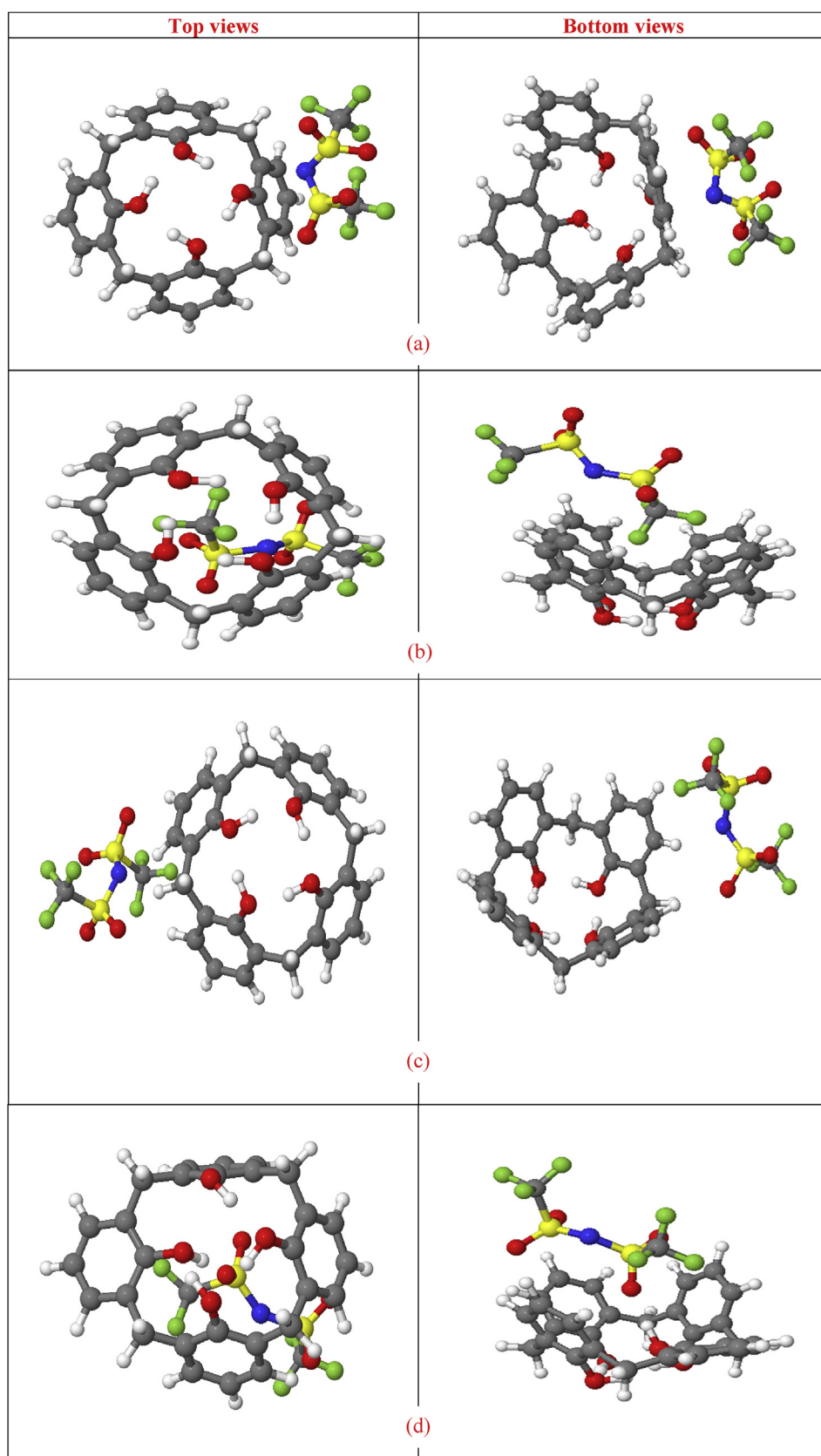
Fig. 1. Optimized geometries of and CX[4]-TFSI - (CX[4]-TFSI - 1 (a), CX[4]-TFSI - 2 (b), CX[4]-TFSI - 3 (c), CX[4]-TFSI - 4 (d)) (Top views and Bottom views) structures using B3LYP-D3/6-31+G(d) method.
