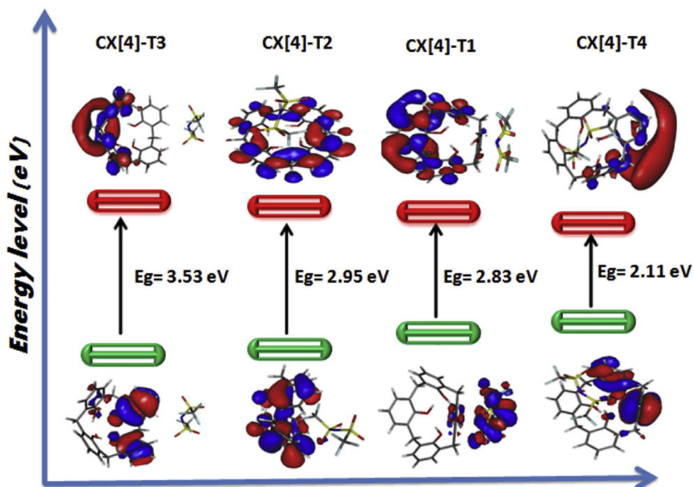
Fig. 3. Frontier Molecular Orbital analysis of CX[4]-TFSI - (CX[4]-T) complexes.
