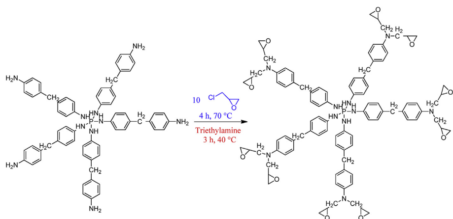
Scheme 2. Synthesis of epoxy polymer DGPMMDAP.
