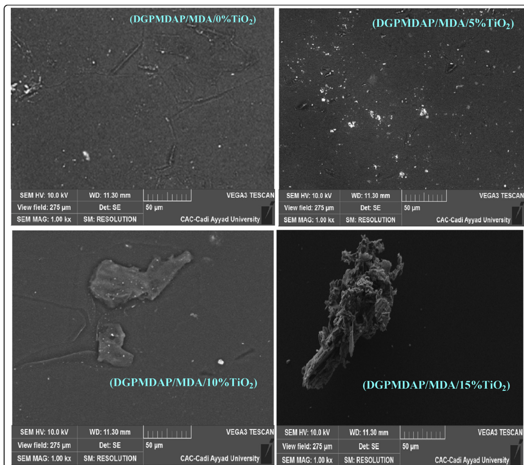
Fig. 8. Morphology of different composite (DGPM DAP/MDA/TiO 2 ) at various percentages (0, 5, 10 and 15%) of TiO 2 .
