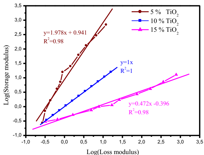
Fig. 7. Cole-Cole chart for composite (DGPM DAP/MDA/TiO 2 ) at different formulation.
