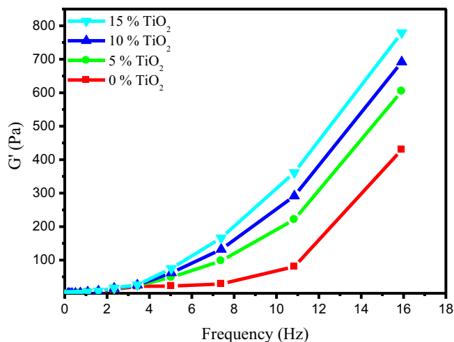
Fig. 5. G' as function of frequency at different composite (DGPMADAP/MDA/TiO 2 ).
