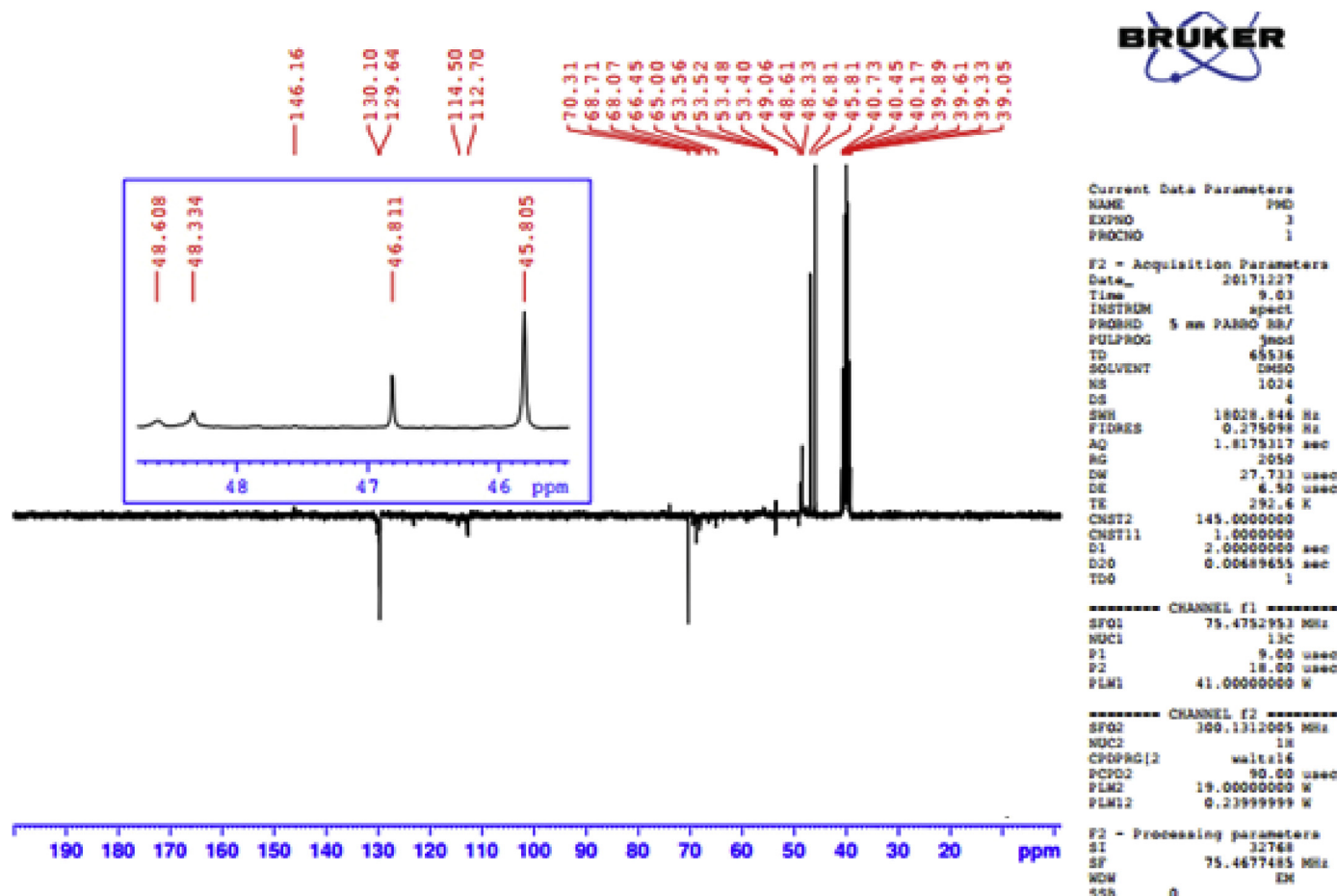
Fig. 3. ^{13}\text{C} NMR spectrum of DGPMADAP.
