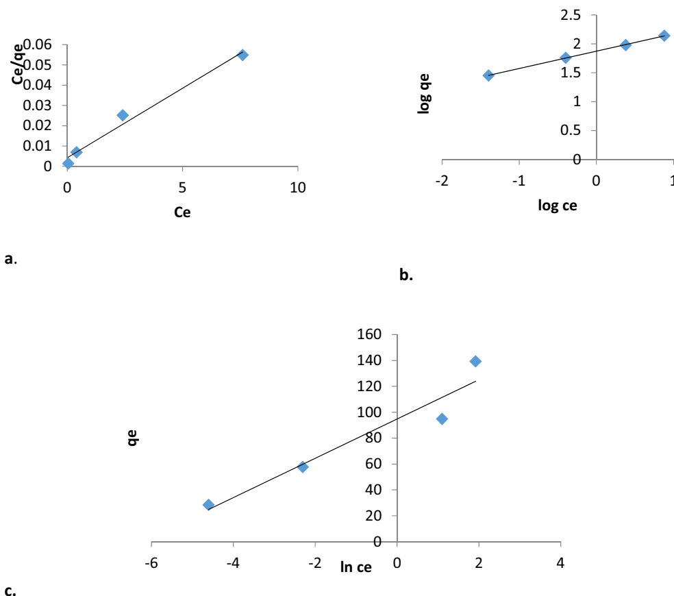
Fig. 8. Plots for (a) Langmuir, (b) Freundlich and (c) Temkin isotherms for \text{Pb}^{2+} adsorption on acid activated Aloji clay at 30 °C.
