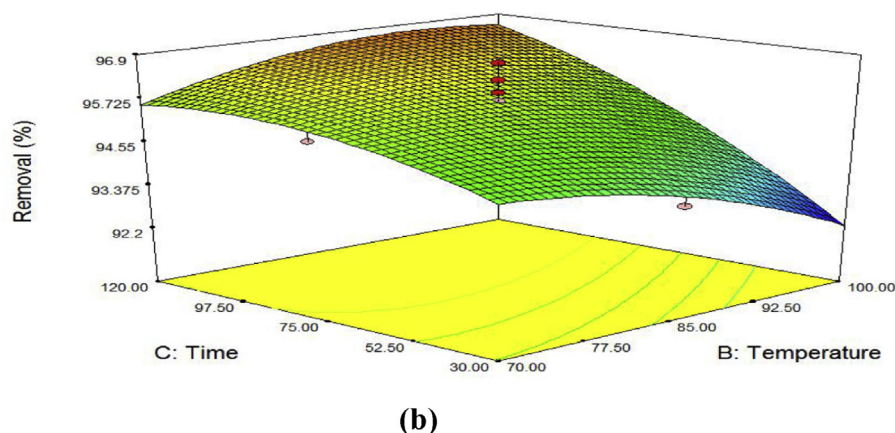
Fig. 3. Effect of activation time and temperature on percentage (a) yield and (b) \text{Pb}^{2+} removal on HCl activated Aloji clay (constant acid activation = 2.25 M).
