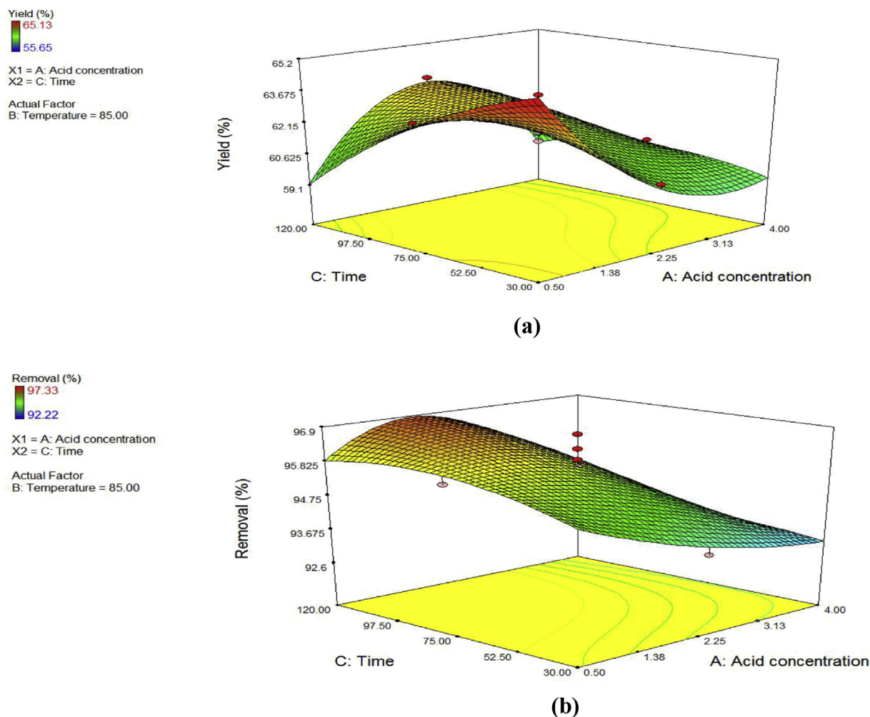
Fig. 2. Acid concentration and time effect on percentage (a) yield and (b) Pb^{2+} removal on HCl activated Aloji clay (constant activation temperature 85 °C).
