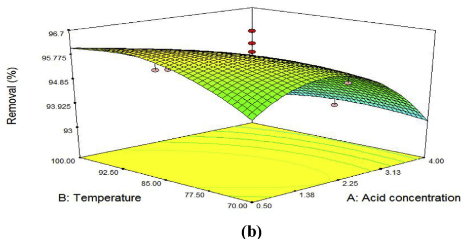
Fig. 1. Effect of acid concentration and temperature on percentage (a) yield and (b) \text{Pb}^{2+} removal on HCl activated Aloji clay (constant time = 75 min).
