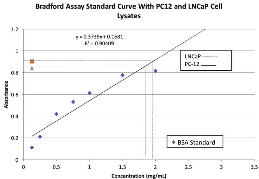
Fig. 2. Protein totals in each lysate via Bradford Assay.
