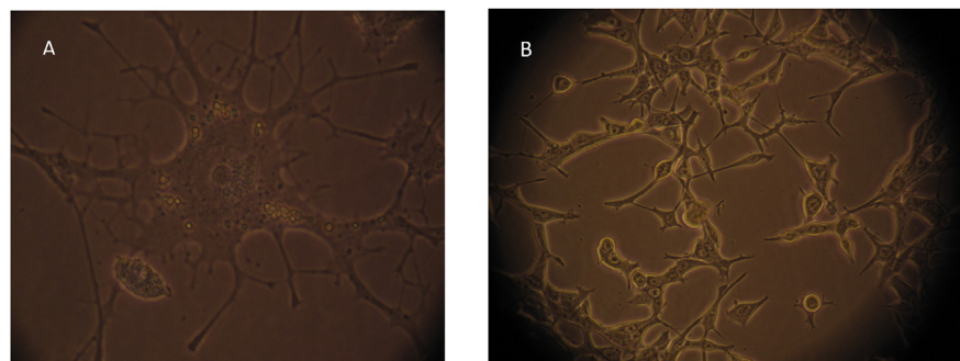
Fig. 1. PC-12 and LNCaP cells in culture. (A) PC-12 cells, at 1000 \times , in 10% FBS-DMEM, supplemented with NGF. (B) LNCaP, at 200 \times , cells grown in 10% FBS-DMEM.
