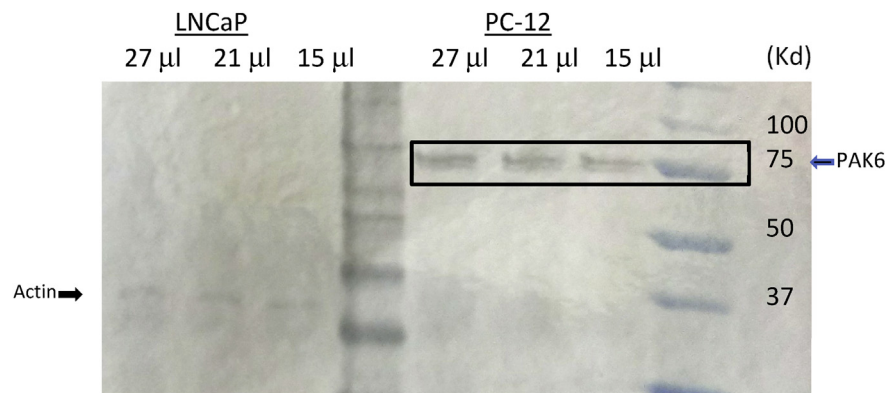
Fig. 3. PAK6 in PC-12, but not LNCaP cells grown in FBS-DMEM.
