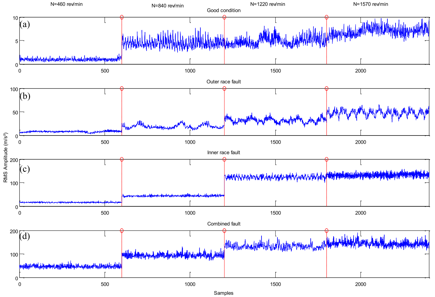
Fig. 6. Results of acquired vibrations for different bearing states and different speeds: (a) healthy, (b) outer race fault, (c) inner race fault, (d) combined defect.
