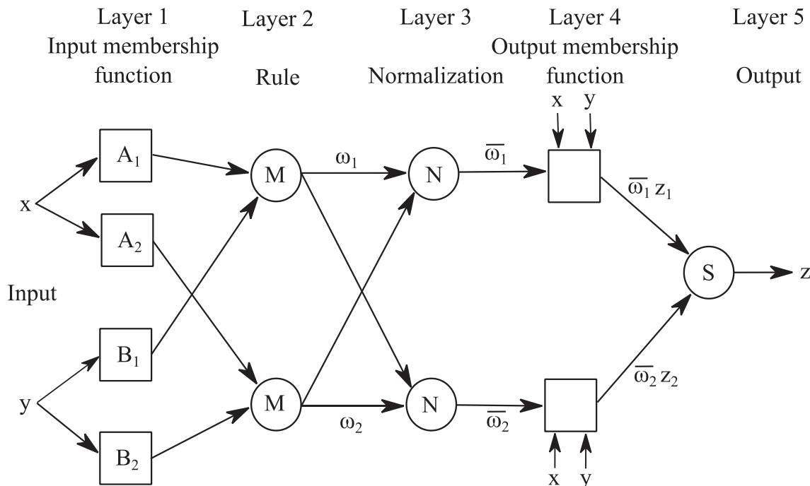
Fig. 1. ANFIS architecture.
