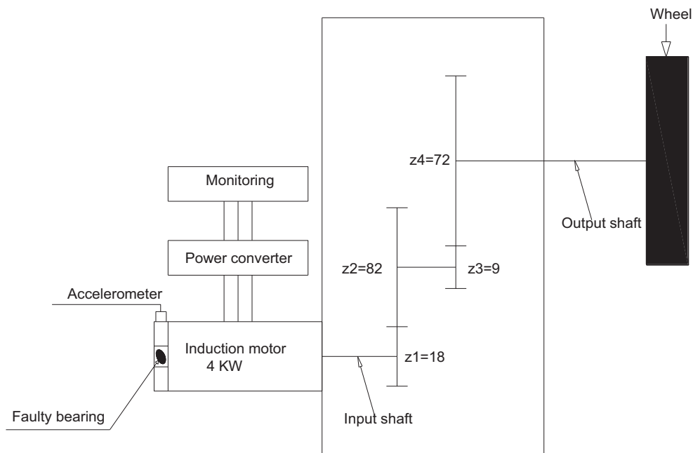
Fig. 3. Kinematic chain of the geared motor.
