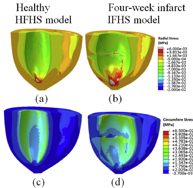
Fig. 4. Contour plots of end-diastolic stress in long axis of the 3D rat heart model of the healthy and remodelling (four-week model) heart models. (a)–(b): Radial stress and (c)–(d): Circumferential stress.
